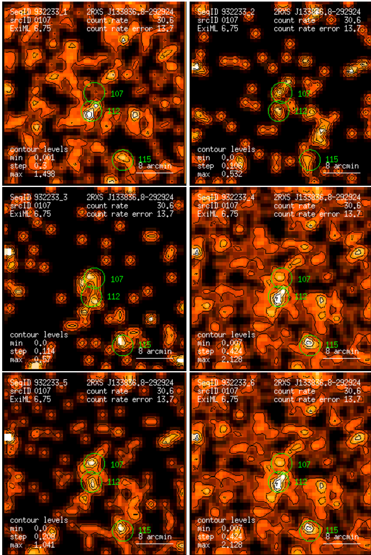
Figure 107: RASS 932233: detection 0107: band rate images, Gaussian filter: (1) PSPC channels 11 – 41, (2) 52 – 90, (3) 91 – 201, (4) 11 – 235, (5) 52 – 201, (6) 11 – 201. Broad band rates in counts/ks. Band rate contour levels in counts/ks/arcmin 2 .
