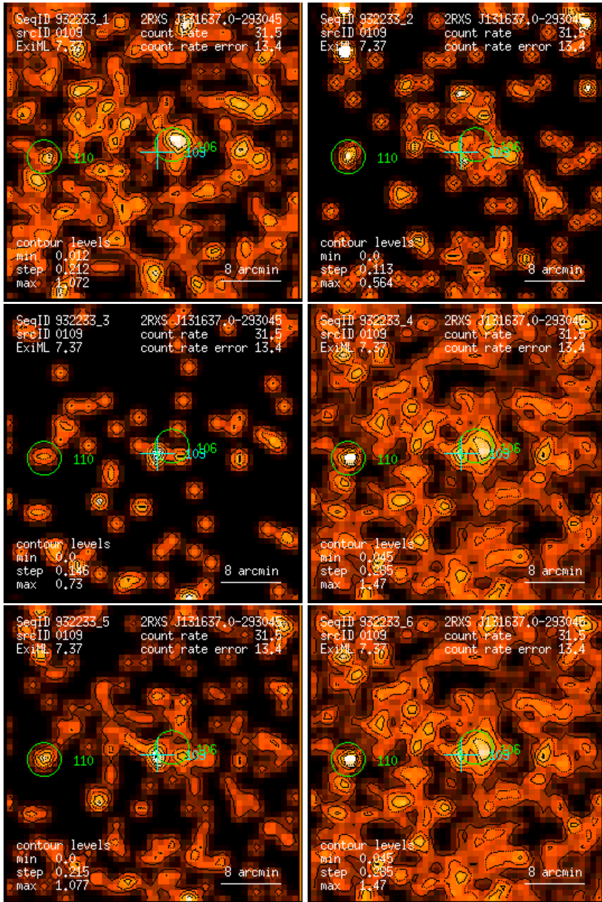
Figure 109: RASS 932233: detection 0109: band rate images, Gaussian filter: (1) PSPC channels 11 – 41, (2) 52 – 90, (3) 91 – 201, (4) 11 – 235, (5) 52 – 201, (6) 11 – 201. Broad band rates in counts/ks. Band rate contour levels in counts/ks/arcmin 2 .
