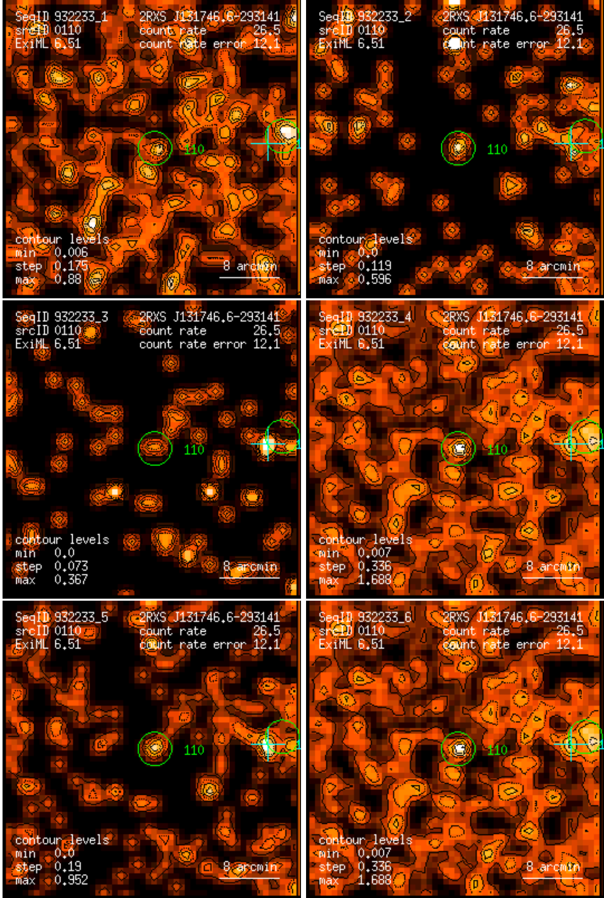
Figure 110: RASS 932233: detection 0110: band rate images, Gaussian filter: (1) PSPC channels 11 – 41, (2) 52 – 90, (3) 91 – 201, (4) 11 – 235, (5) 52 – 201, (6) 11 – 201. Broad band rates in counts/ks. Band rate contour levels in counts/ks/arcmin 2 .
