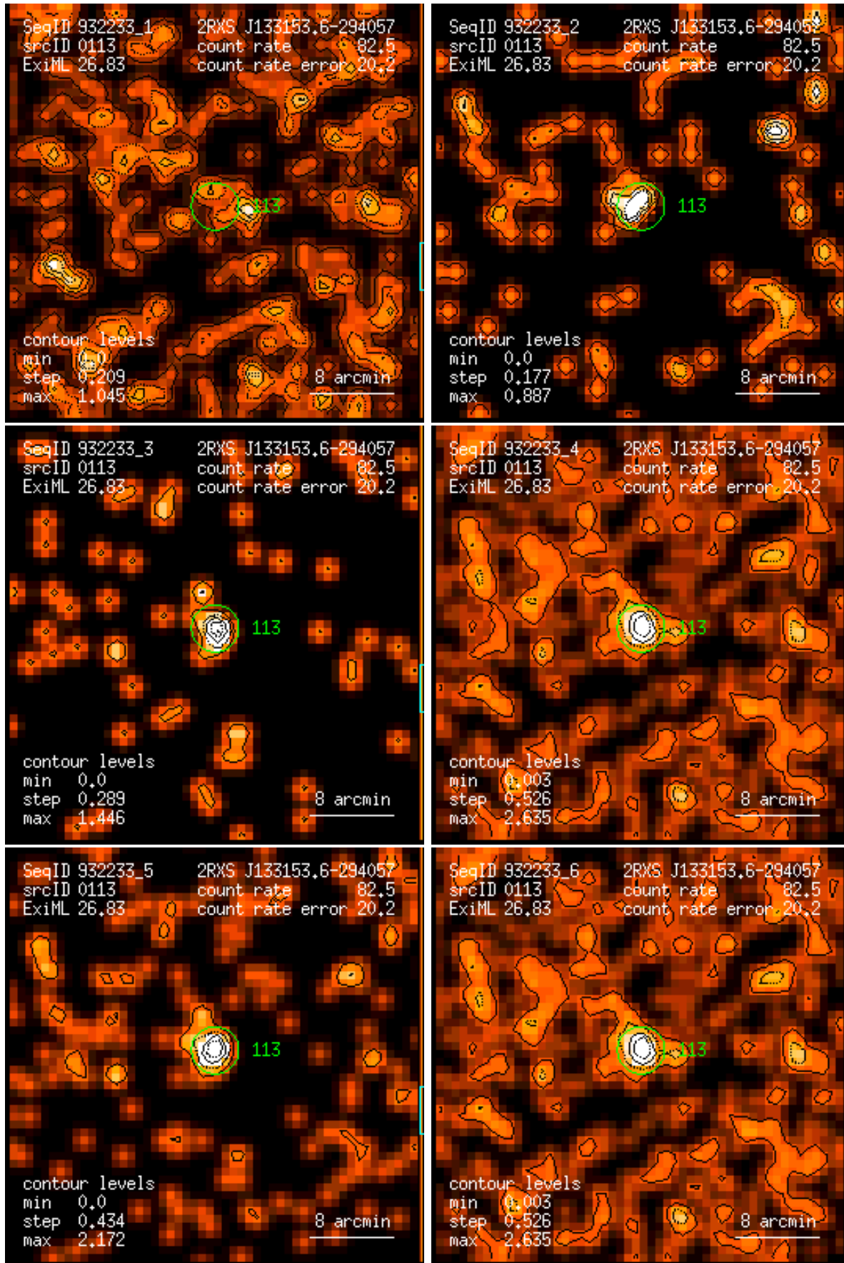
Figure 113: RASS 932233: detection 0113: band rate images, Gaussian filter: (1) PSPC channels 11 – 41, (2) 52 – 90, (3) 91 – 201, (4) 11 – 235, (5) 52 – 201, (6) 11 – 201. Broad band rates in counts/ks. Band rate contour levels in counts/ks/arcmin 2 .
