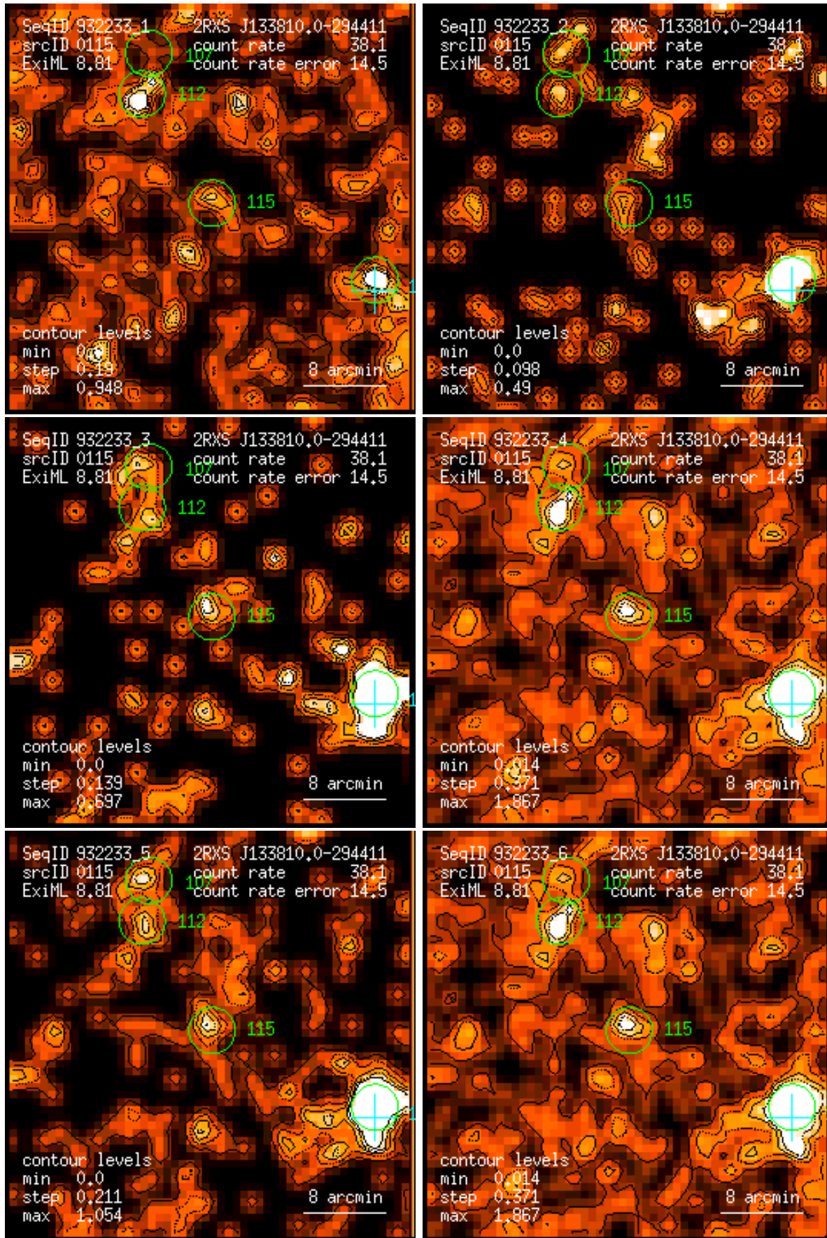
Figure 115: RASS 932233: detection 0115: band rate images, Gaussian filter: (1) PSPC channels 11 – 41, (2) 52 – 90, (3) 91 – 201, (4) 11 – 235, (5) 52 – 201, (6) 11 – 201. Broad band rates in counts/ks. Band rate contour levels in counts/ks/arcmin 2 .
