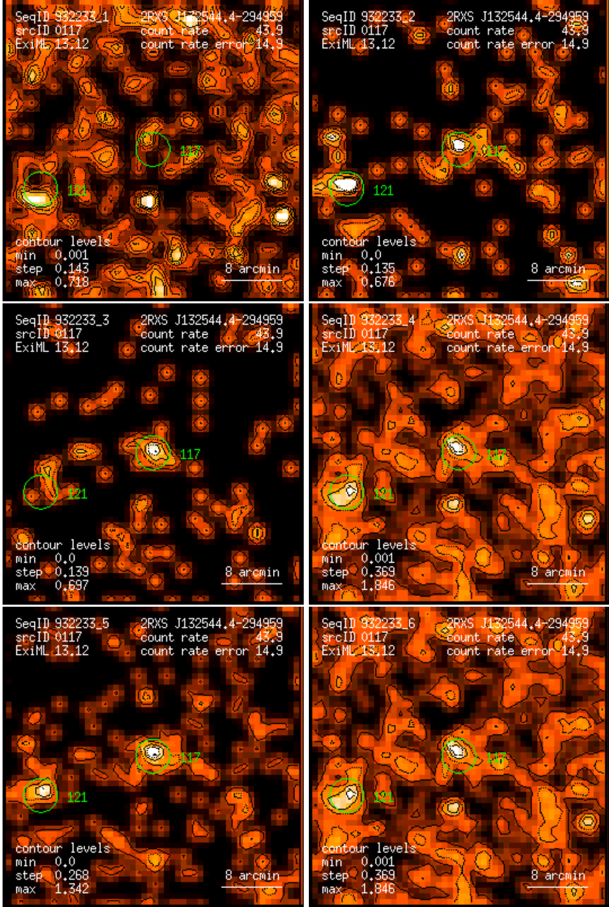
Figure 117: RASS 932233: detection 0117: band rate images, Gaussian filter: (1) PSPC channels 11 – 41, (2) 52 – 90, (3) 91 – 201, (4) 11 – 235, (5) 52 – 201, (6) 11 – 201. Broad band rates in counts/ks. Band rate contour levels in counts/ks/arcmin 2 .
