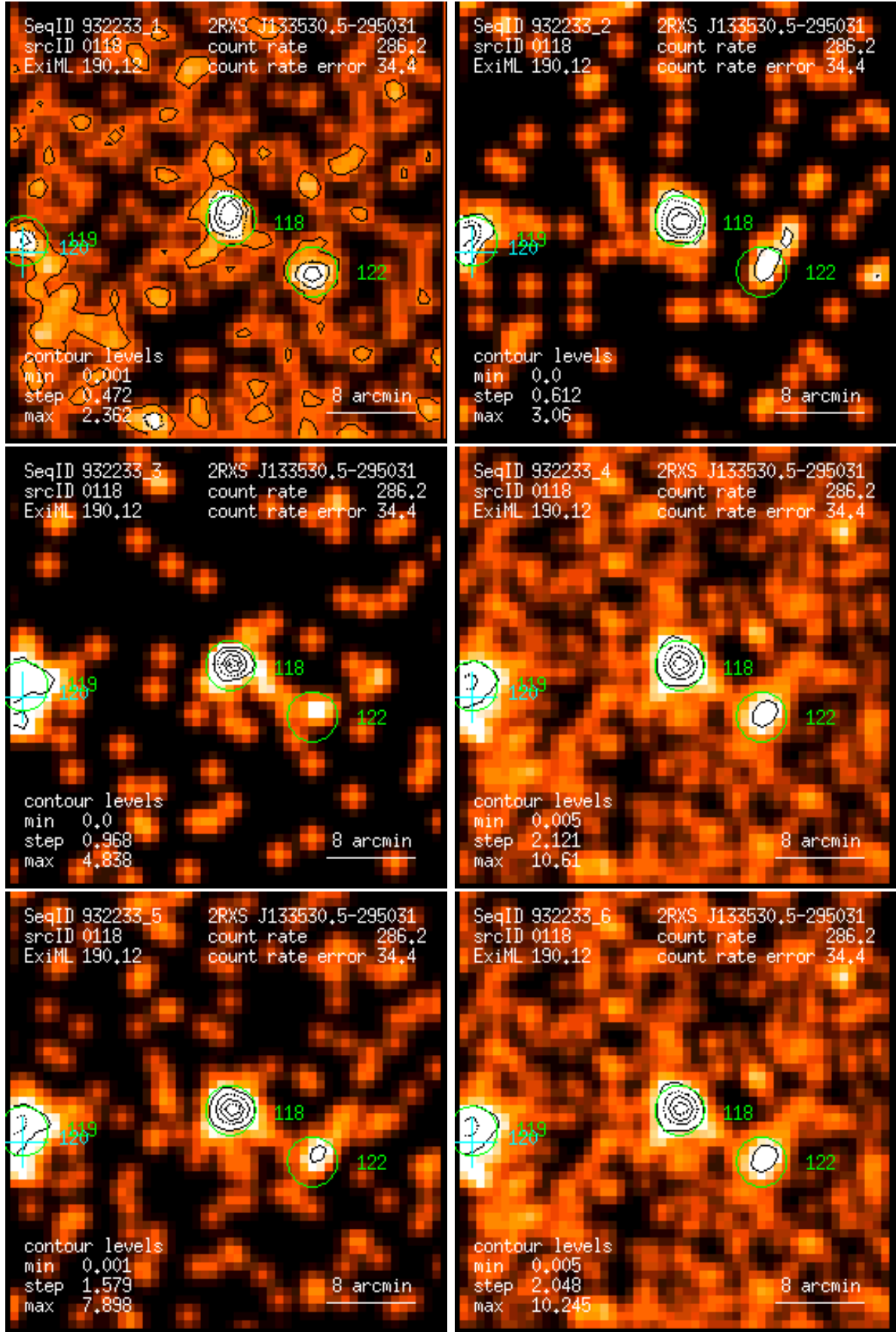
Figure 118: RASS 932233: detection 0118: band rate images, Gaussian filter: (1) PSPC channels 11 – 41, (2) 52 – 90, (3) 91 – 201, (4) 11 – 235, (5) 52 – 201, (6) 11 – 201. Broad band rates in counts/ks. Band rate contour levels in counts/ks/arcmin 2 .
