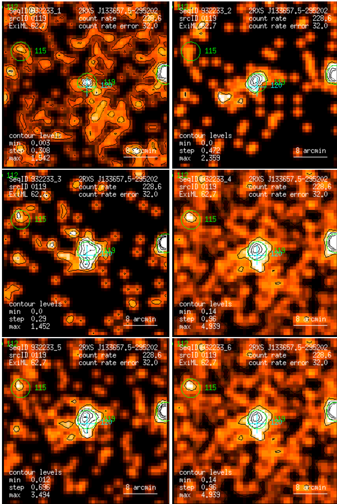
Figure 119: RASS 932233: detection 0119: band rate images, Gaussian filter: (1) PSPC channels 11 – 41, (2) 52 – 90, (3) 91 – 201, (4) 11 – 235, (5) 52 – 201, (6) 11 – 201. Broad band rates in counts/ks. Band rate contour levels in counts/ks/arcmin 2 .
