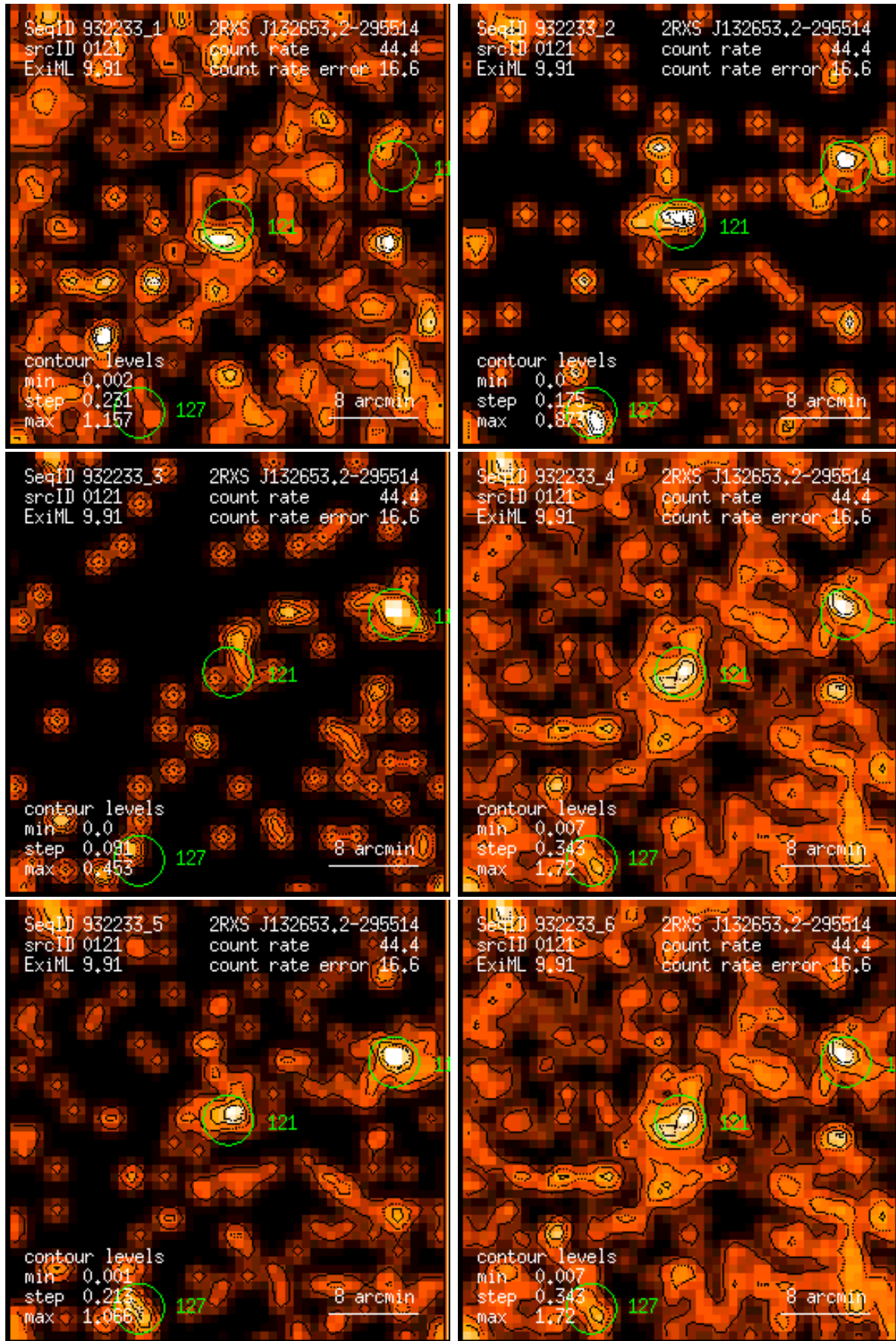
Figure 121: RASS 932233: detection 0121: band rate images, Gaussian filter: (1) PSPC channels 11 – 41, (2) 52 – 90, (3) 91 – 201, (4) 11 – 235, (5) 52 – 201, (6) 11 – 201. Broad band rates in counts/ks. Band rate contour levels in counts/ks/arcmin 2 .
