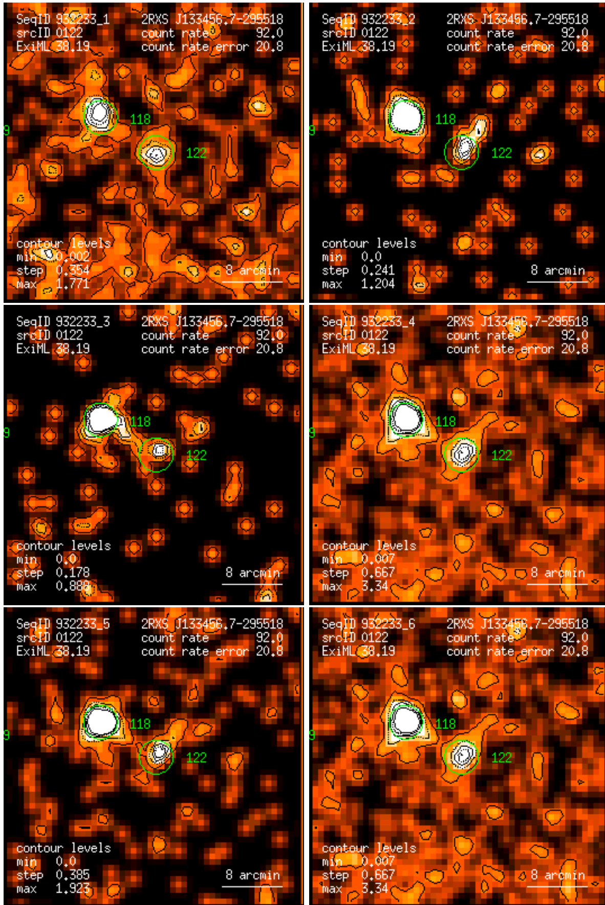
Figure 122: RASS 932233: detection 0122: band rate images, Gaussian filter: (1) PSPC channels 11 – 41, (2) 52 – 90, (3) 91 – 201, (4) 11 – 235, (5) 52 – 201, (6) 11 – 201. Broad band rates in counts/ks. Band rate contour levels in counts/ks/arcmin 2 .
