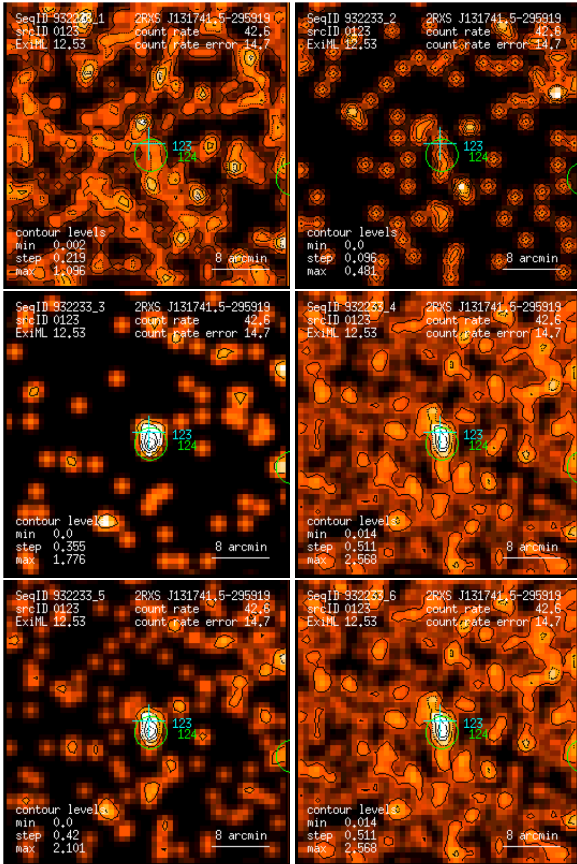
Figure 123: RASS 932233: detection 0123: band rate images, Gaussian filter: (1) PSPC channels 11 – 41, (2) 52 – 90, (3) 91 – 201, (4) 11 – 235, (5) 52 – 201, (6) 11 – 201. Broad band rates in counts/ks. Band rate contour levels in counts/ks/arcmin 2 .
