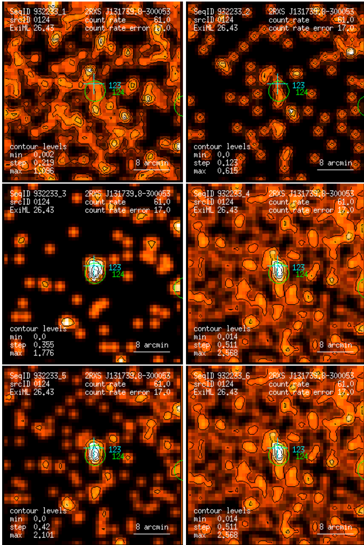
Figure 124: RASS 932233: detection 0124: band rate images, Gaussian filter: (1) PSPC channels 11 – 41, (2) 52 – 90, (3) 91 – 201, (4) 11 – 235, (5) 52 – 201, (6) 11 – 201. Broad band rates in counts/ks. Band rate contour levels in counts/ks/arcmin 2 .
