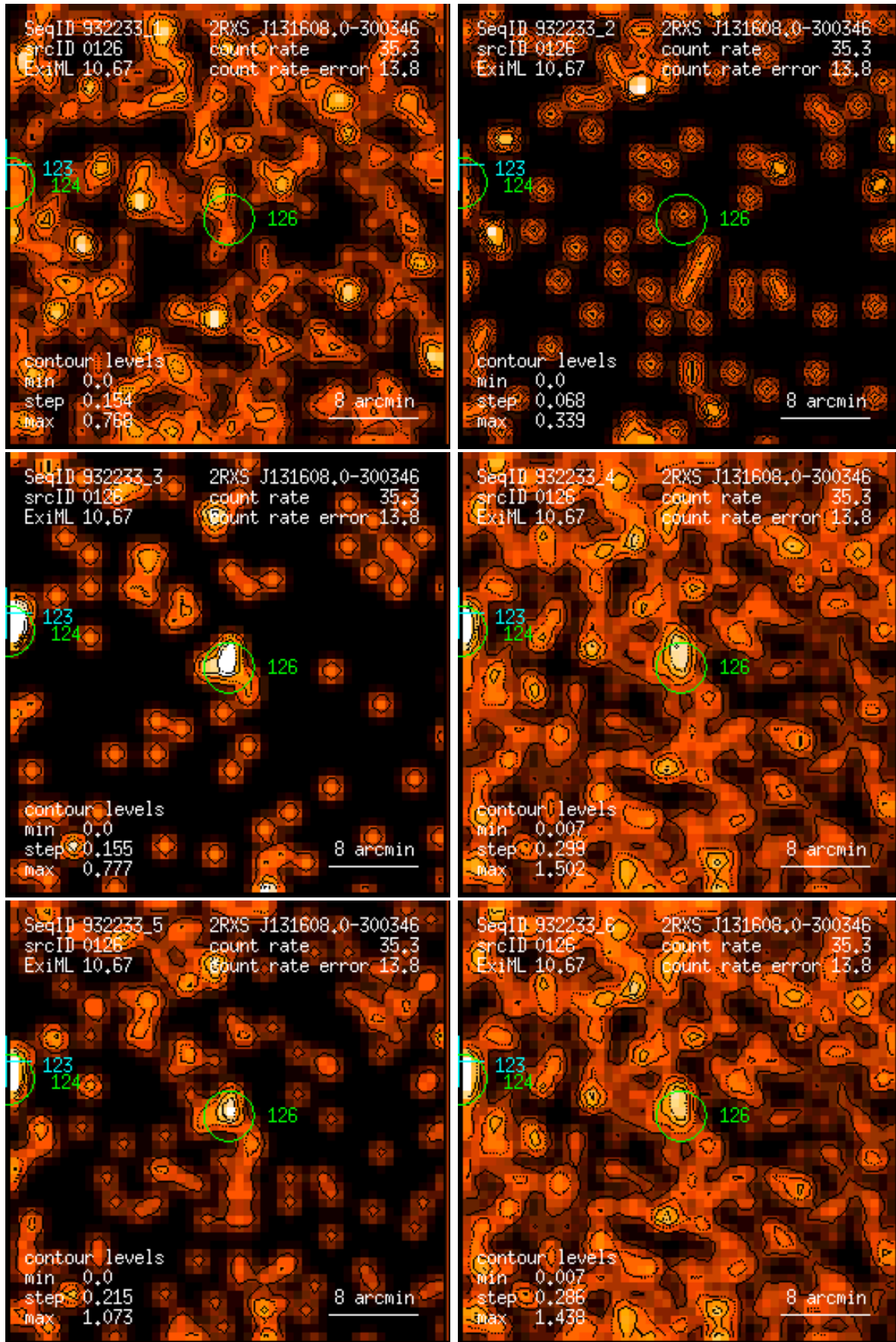
Figure 126: RASS 932233: detection 0126: band rate images, Gaussian filter: (1) PSPC channels 11 – 41, (2) 52 – 90, (3) 91 – 201, (4) 11 – 235, (5) 52 – 201, (6) 11 – 201. Broad band rates in counts/ks. Band rate contour levels in counts/ks/arcmin 2 .
