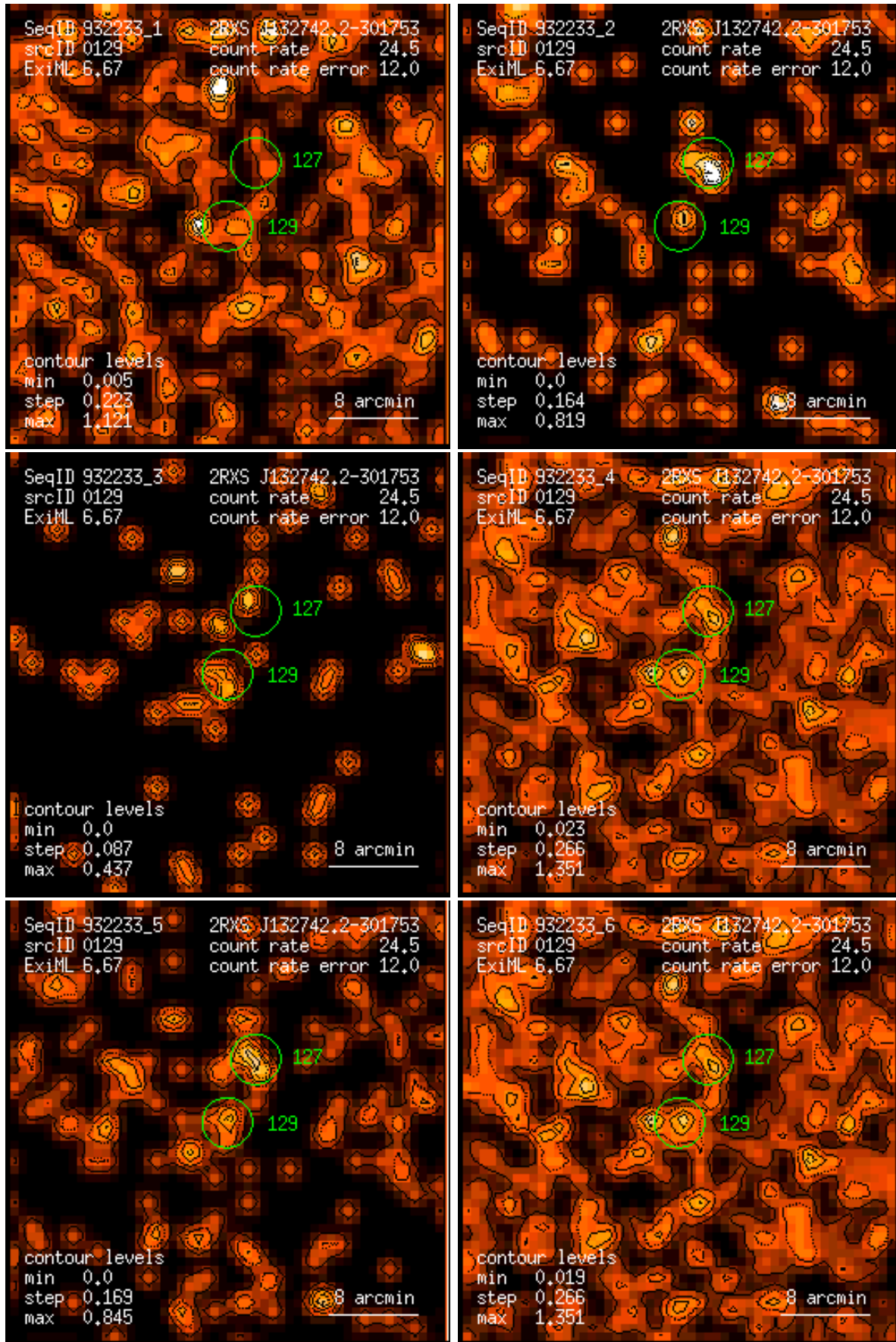
Figure 129: RASS 932233: detection 0129: band rate images, Gaussian filter: (1) PSPC channels 11 – 41, (2) 52 – 90, (3) 91 – 201, (4) 11 – 235, (5) 52 – 201, (6) 11 – 201. Broad band rates in counts/ks. Band rate contour levels in counts/ks/arcmin 2 .
