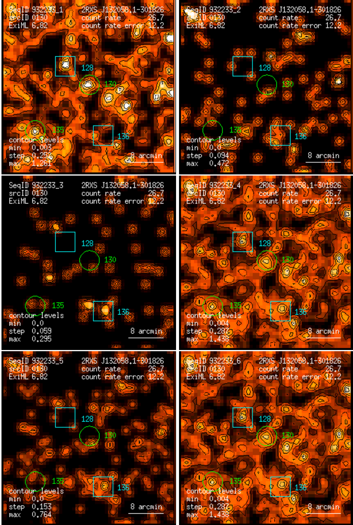
Figure 130: RASS 932233: detection 0130: band rate images, Gaussian filter: (1) PSPC channels 11 – 41, (2) 52 – 90, (3) 91 – 201, (4) 11 – 235, (5) 52 – 201, (6) 11 – 201. Broad band rates in counts/ks. Band rate contour levels in counts/ks/arcmin 2 .
