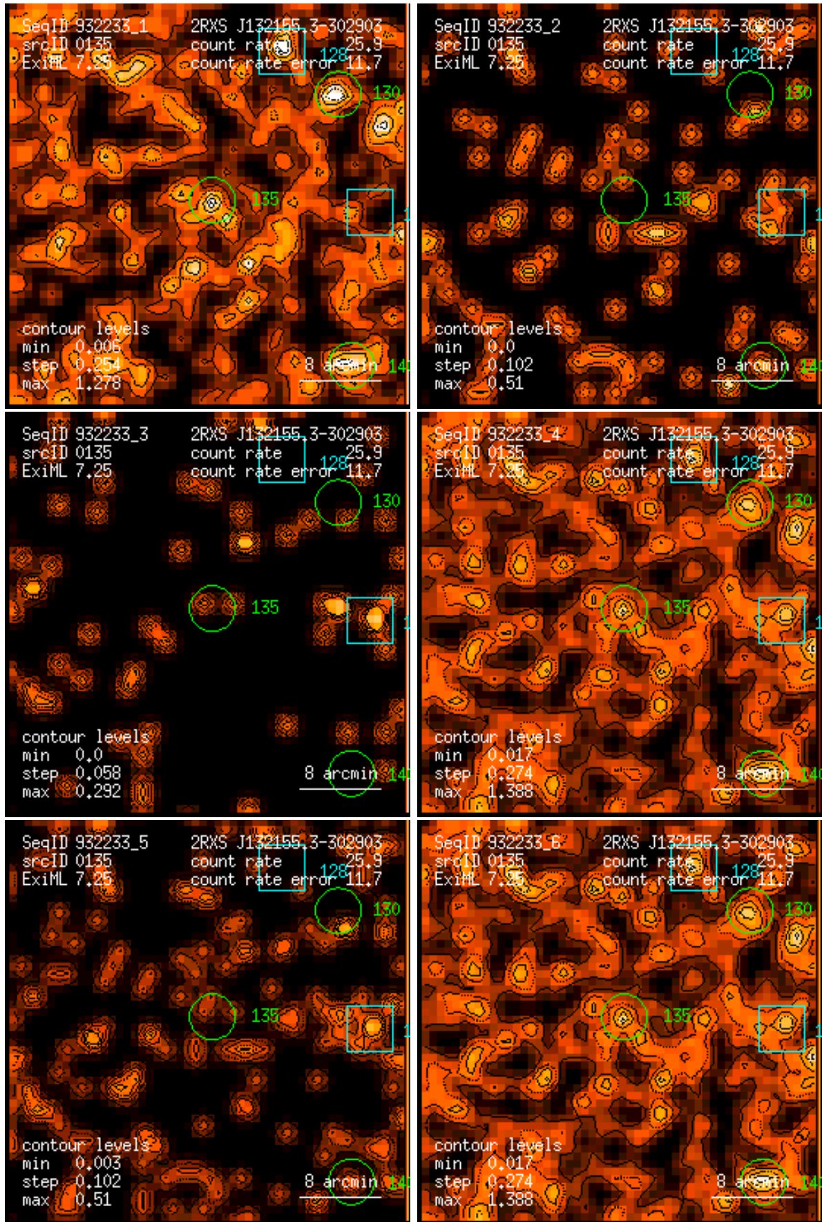
Figure 135: RASS 932233: detection 0135: band rate images, Gaussian filter: (1) PSPC channels 11 – 41, (2) 52 – 90, (3) 91 – 201, (4) 11 – 235, (5) 52 – 201, (6) 11 – 201. Broad band rates in counts/ks. Band rate contour levels in counts/ks/arcmin 2 .
