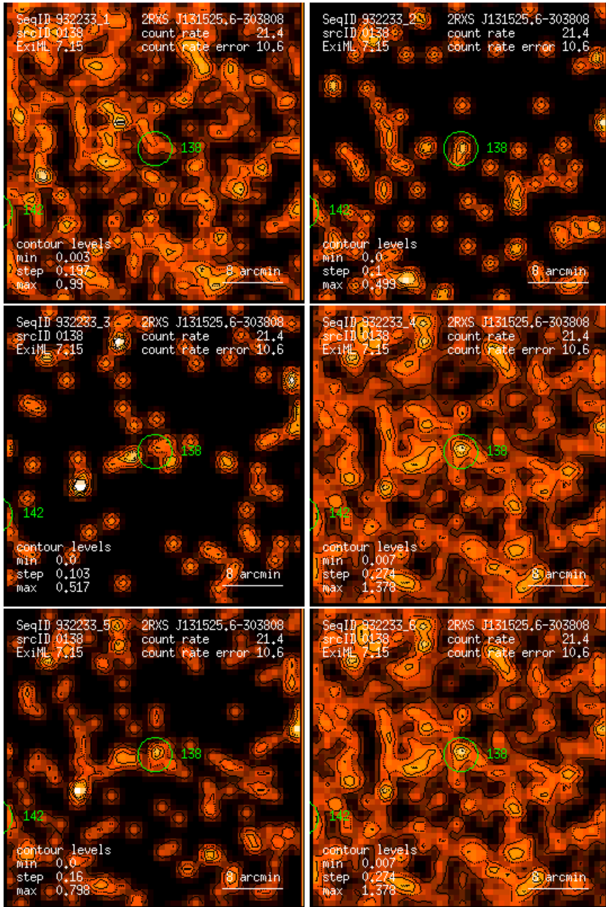
Figure 138: RASS 932233: detection 0138: band rate images, Gaussian filter: (1) PSPC channels 11 – 41, (2) 52 – 90, (3) 91 – 201, (4) 11 – 235, (5) 52 – 201, (6) 11 – 201. Broad band rates in counts/ks. Band rate contour levels in counts/ks/arcmin 2 .
