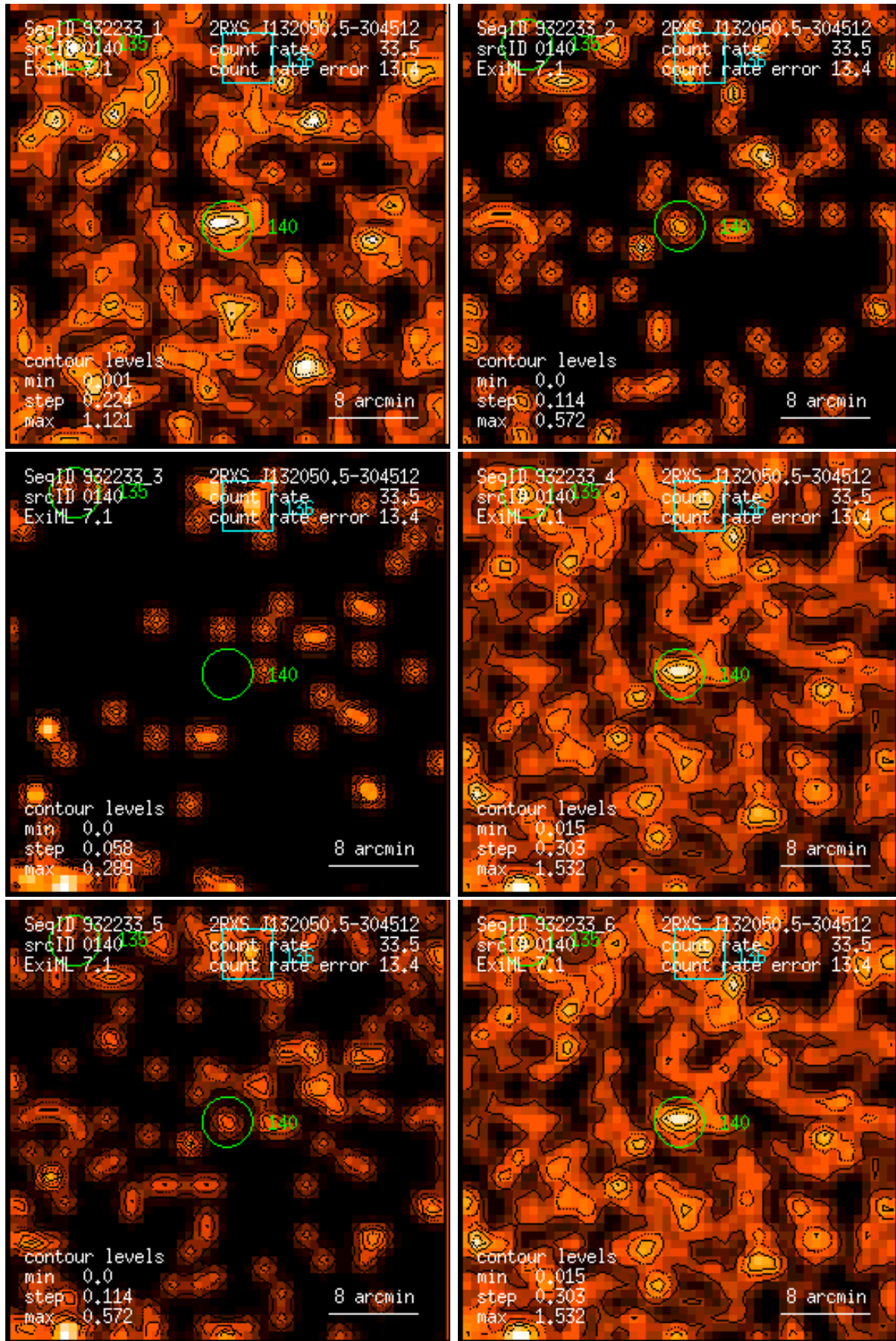
Figure 140: RASS 932233: detection 0140: band rate images, Gaussian filter: (1) PSPC channels 11 – 41, (2) 52 – 90, (3) 91 – 201, (4) 11 – 235, (5) 52 – 201, (6) 11 – 201. Broad band rates in counts/ks. Band rate contour levels in counts/ks/arcmin 2 .
