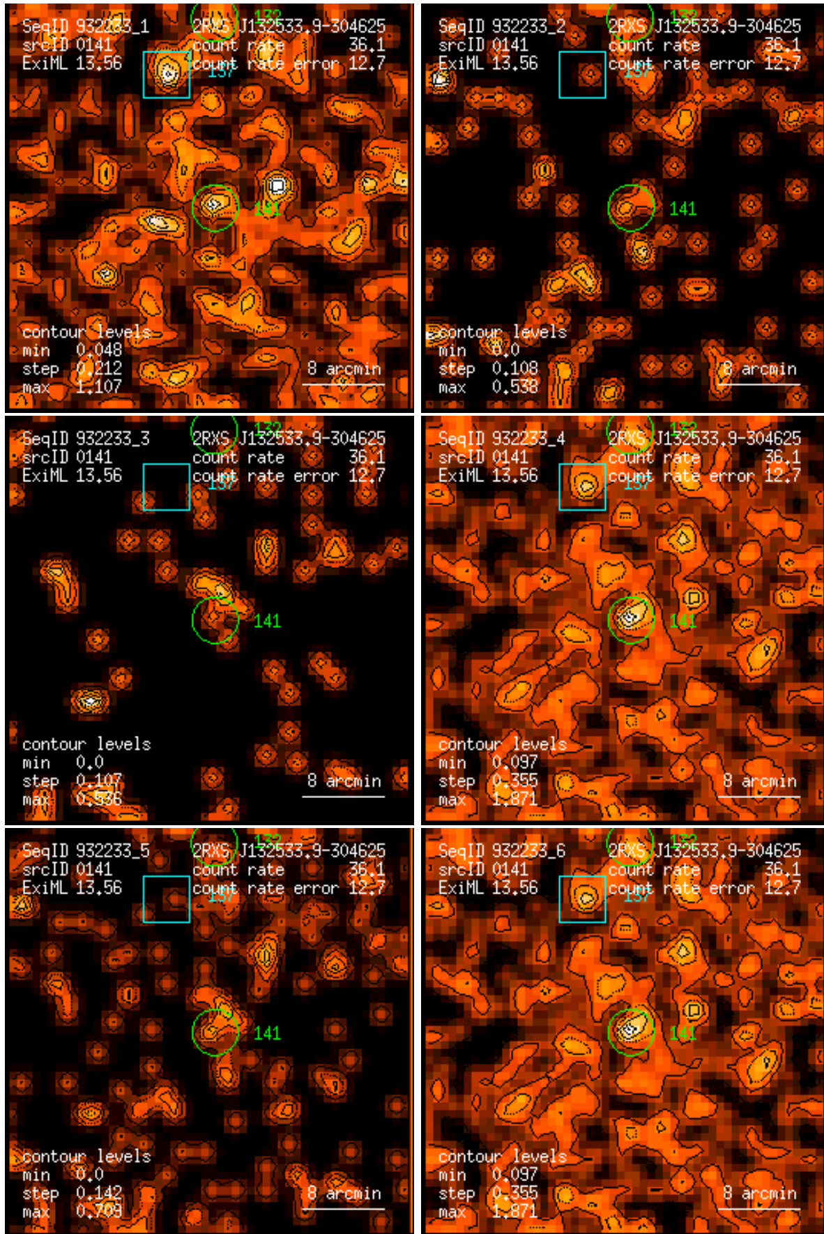
Figure 141: RASS 932233: detection 0141: band rate images, Gaussian filter: (1) PSPC channels 11 – 41, (2) 52 – 90, (3) 91 – 201, (4) 11 – 235, (5) 52 – 201, (6) 11 – 201. Broad band rates in counts/ks. Band rate contour levels in counts/ks/arcmin 2 .
