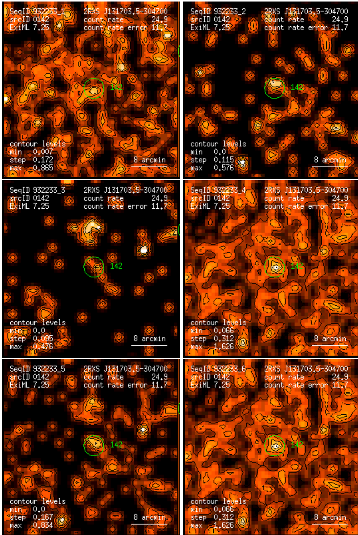
Figure 142: RASS 932233: detection 0142: band rate images, Gaussian filter: (1) PSPC channels 11 – 41, (2) 52 – 90, (3) 91 – 201, (4) 11 – 235, (5) 52 – 201, (6) 11 – 201. Broad band rates in counts/ks. Band rate contour levels in counts/ks/arcmin 2 .
