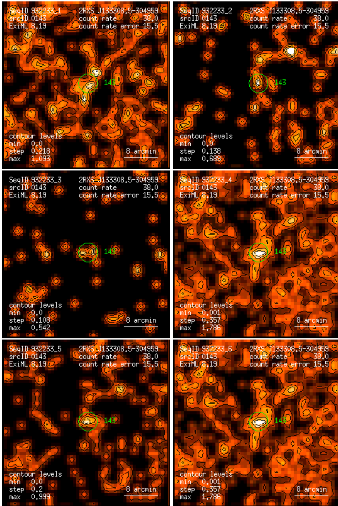
Figure 143: RASS 932233: detection 0143: band rate images, Gaussian filter: (1) PSPC channels 11 – 41, (2) 52 – 90, (3) 91 – 201, (4) 11 – 235, (5) 52 – 201, (6) 11 – 201. Broad band rates in counts/ks. Band rate contour levels in counts/ks/arcmin 2 .
