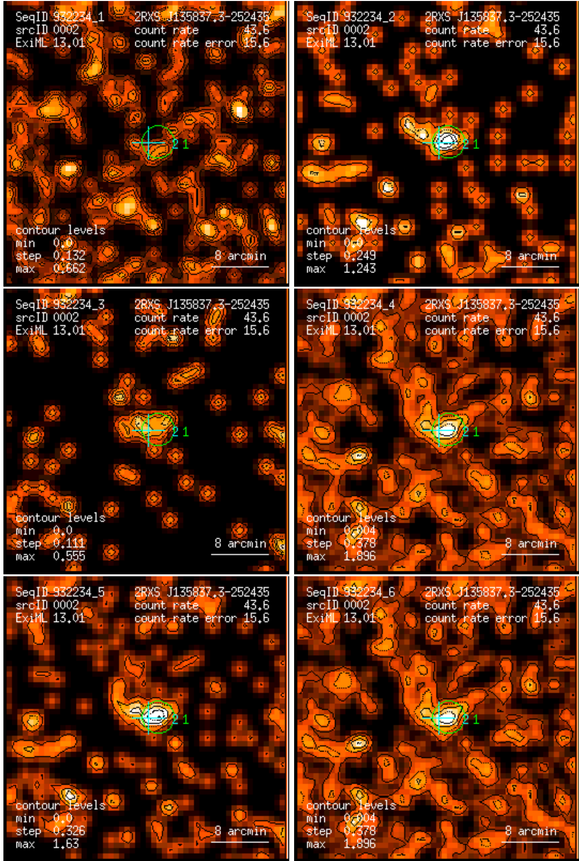
Figure 2: RASS 932234: detection 0002: band rate images, Gaussian filter: (1) PSPC channels 11 – 41, (2) 52 – 90, (3) 91 – 201, (4) 11 – 235, (5) 52 – 201, (6) 11 – 201. Broad band rates in counts/ks. Band rate contour levels in counts/ks/arcmin 2 .
