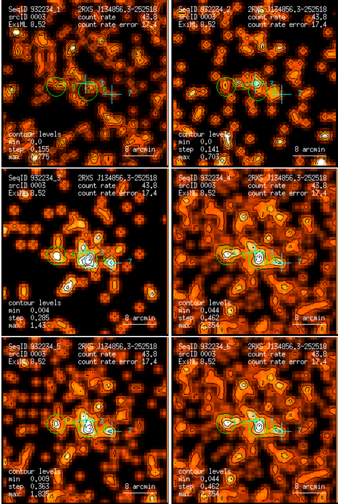
Figure 3: RASS 932234: detection 0003: band rate images, Gaussian filter: (1) PSPC channels 11 – 41, (2) 52 – 90, (3) 91 – 201, (4) 11 – 235, (5) 52 – 201, (6) 11 – 201. Broad band rates in counts/ks. Band rate contour levels in counts/ks/arcmin 2 .
