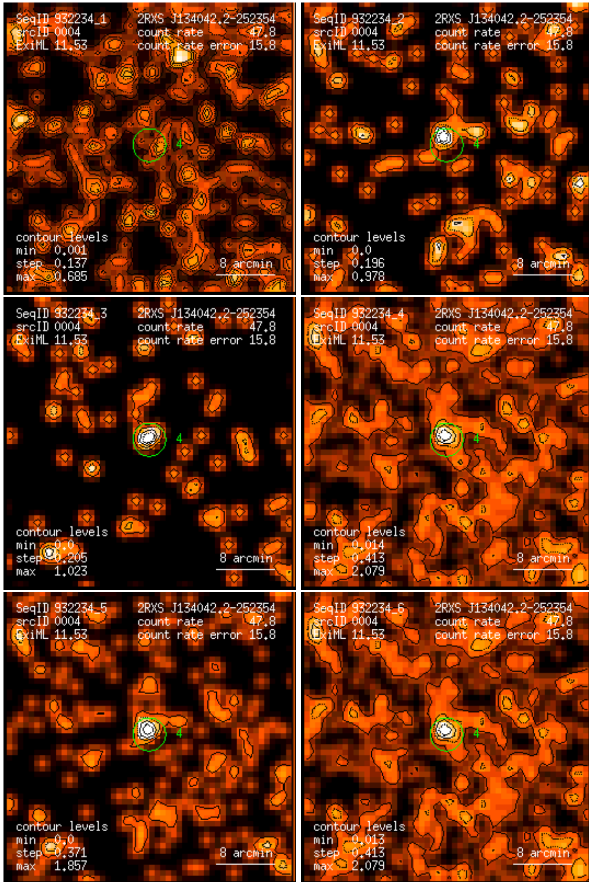
Figure 4: RASS 932234: detection 0004: band rate images, Gaussian filter: (1) PSPC channels 11 – 41, (2) 52 – 90, (3) 91 – 201, (4) 11 – 235, (5) 52 – 201, (6) 11 – 201. Broad band rates in counts/ks. Band rate contour levels in counts/ks/arcmin 2 .
