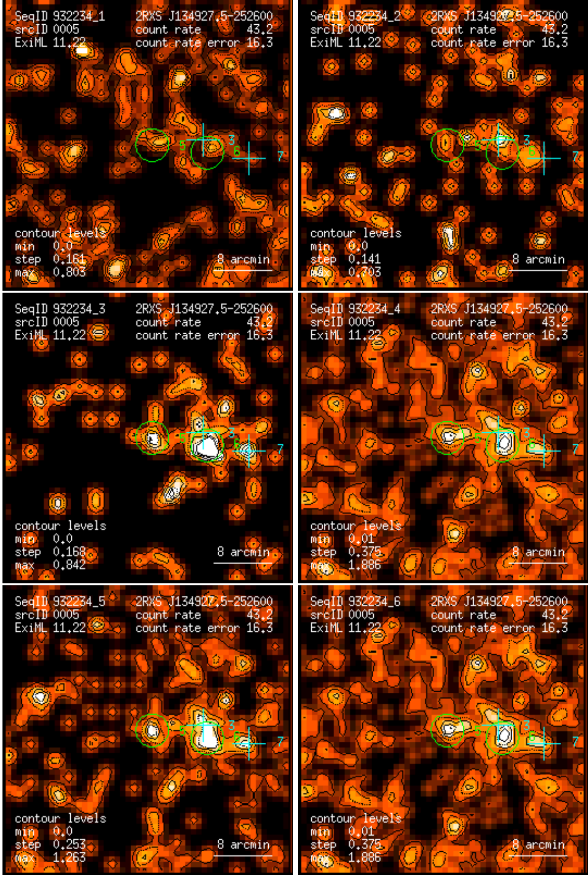
Figure 5: RASS 932234: detection 0005: band rate images, Gaussian filter: (1) PSPC channels 11 – 41, (2) 52 – 90, (3) 91 – 201, (4) 11 – 235, (5) 52 – 201, (6) 11 – 201. Broad band rates in counts/ks. Band rate contour levels in counts/ks/arcmin 2 .
