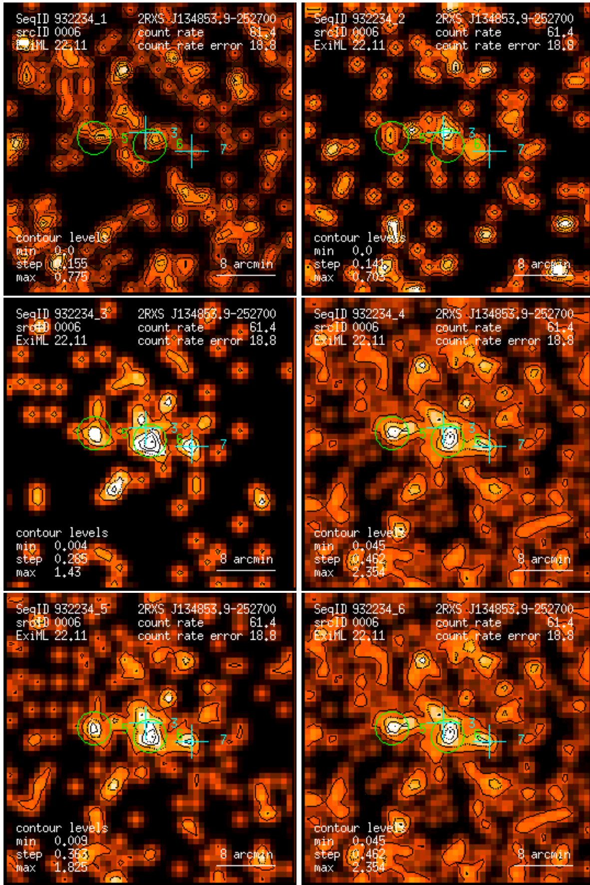
Figure 6: RASS 932234: detection 0006: band rate images, Gaussian filter: (1) PSPC channels 11 – 41, (2) 52 – 90, (3) 91 – 201, (4) 11 – 235, (5) 52 – 201, (6) 11 – 201. Broad band rates in counts/ks. Band rate contour levels in counts/ks/arcmin 2 .
