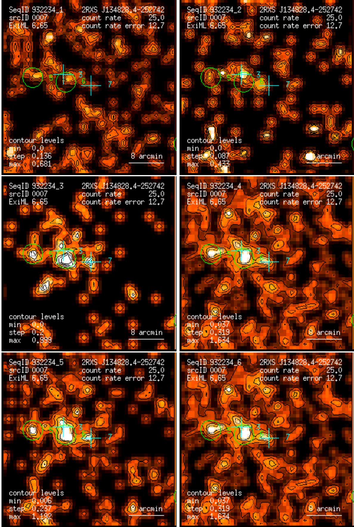
Figure 7: RASS 932234: detection 0007: band rate images, Gaussian filter: (1) PSPC channels 11 – 41, (2) 52 – 90, (3) 91 – 201, (4) 11 – 235, (5) 52 – 201, (6) 11 – 201. Broad band rates in counts/ks. Band rate contour levels in counts/ks/arcmin 2 .
