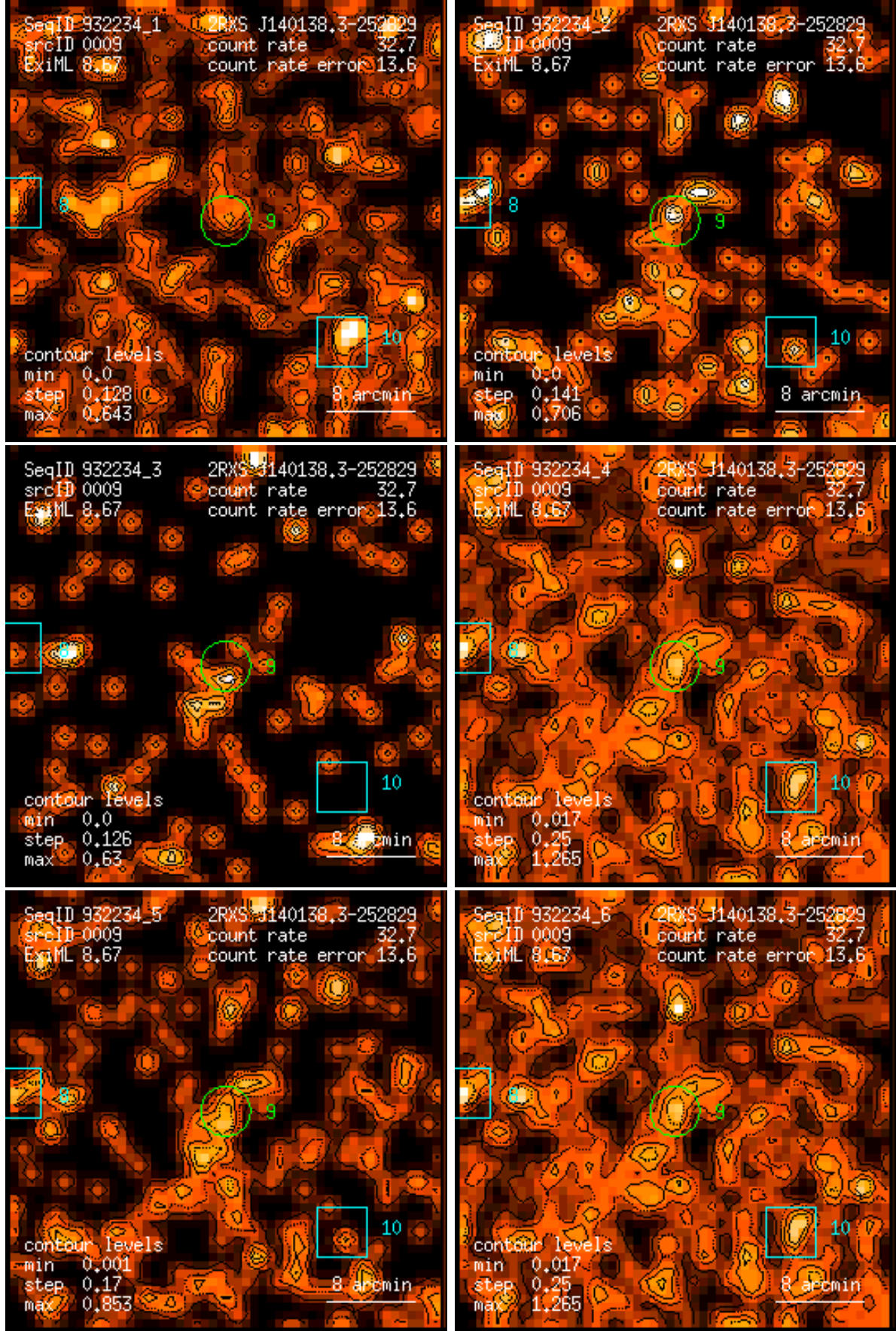
Figure 9: RASS 932234: detection 0009: band rate images, Gaussian filter: (1) PSPC channels 11 – 41, (2) 52 – 90, (3) 91 – 201, (4) 11 – 235, (5) 52 – 201, (6) 11 – 201. Broad band rates in counts/ks. Band rate contour levels in counts/ks/arcmin 2 .
