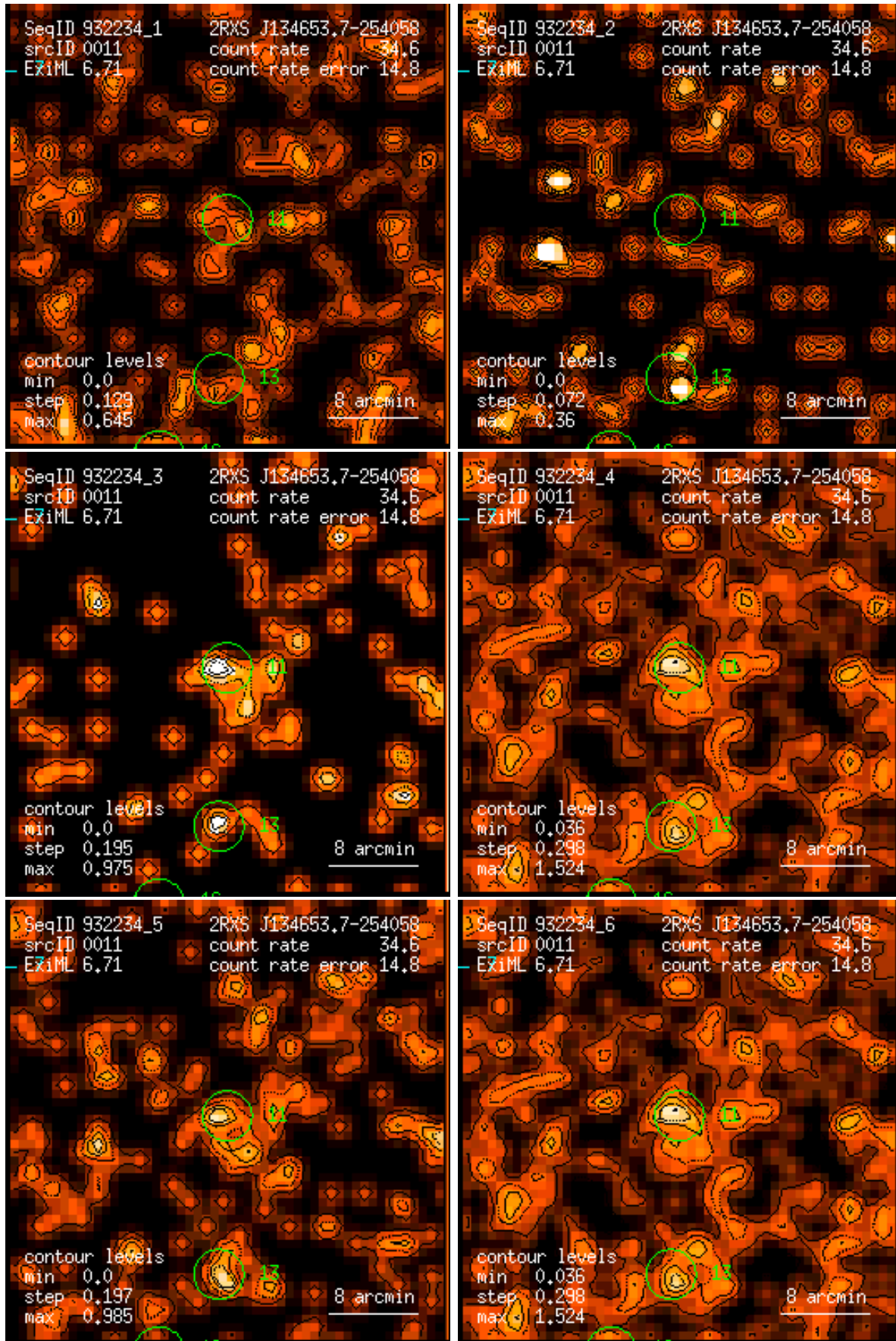
Figure 11: RASS 932234: detection 0011: band rate images, Gaussian filter: (1) PSPC channels 11 – 41, (2) 52 – 90, (3) 91 – 201, (4) 11 – 235, (5) 52 – 201, (6) 11 – 201. Broad band rates in counts/ks. Band rate contour levels in counts/ks/arcmin 2 .
