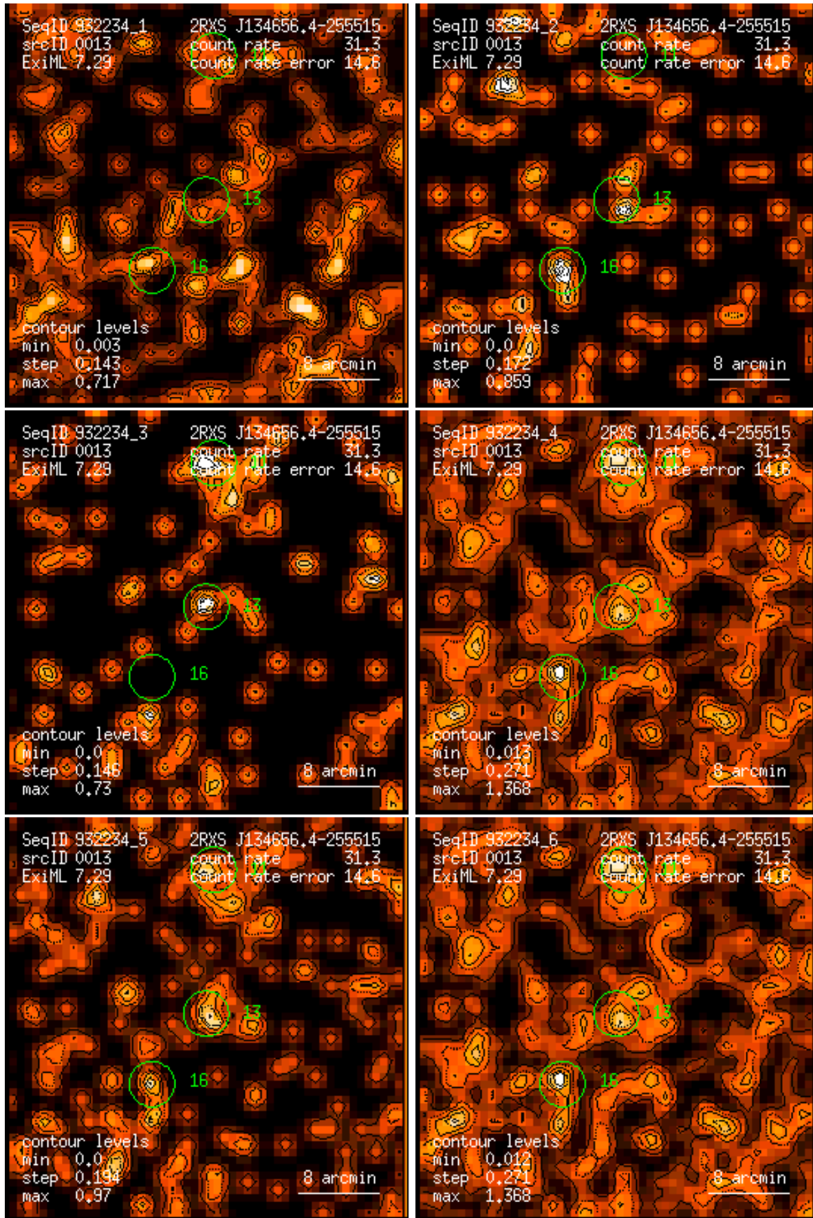
Figure 13: RASS 932234: detection 0013: band rate images, Gaussian filter: (1) PSPC channels 11 – 41, (2) 52 – 90, (3) 91 – 201, (4) 11 – 235, (5) 52 – 201, (6) 11 – 201. Broad band rates in counts/ks. Band rate contour levels in counts/ks/arcmin 2 .
