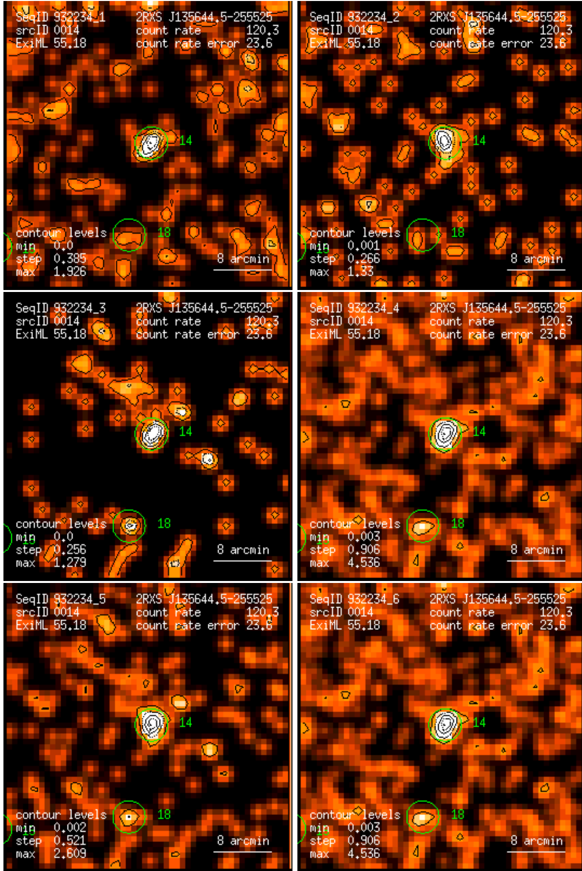
Figure 14: RASS 932234: detection 0014: band rate images, Gaussian filter: (1) PSPC channels 11 – 41, (2) 52 – 90, (3) 91 – 201, (4) 11 – 235, (5) 52 – 201, (6) 11 – 201. Broad band rates in counts/ks. Band rate contour levels in counts/ks/arcmin 2 .
