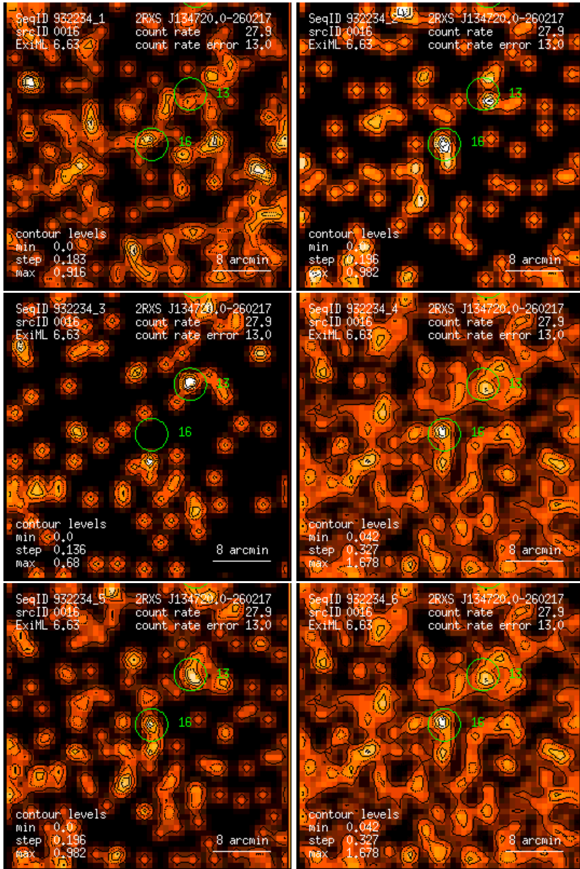
Figure 16: RASS 932234: detection 0016: band rate images, Gaussian filter: (1) PSPC channels 11 – 41, (2) 52 – 90, (3) 91 – 201, (4) 11 – 235, (5) 52 – 201, (6) 11 – 201. Broad band rates in counts/ks. Band rate contour levels in counts/ks/arcmin 2 .
