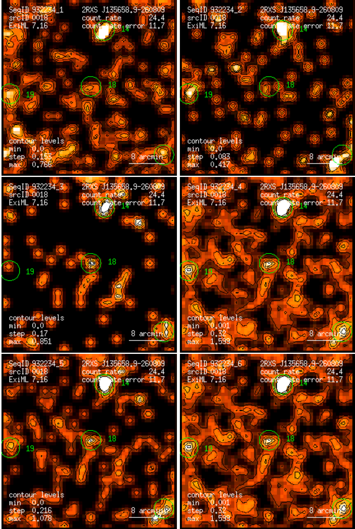
Figure 18: RASS 932234: detection 0018: band rate images, Gaussian filter: (1) PSPC channels 11 – 41, (2) 52 – 90, (3) 91 – 201, (4) 11 – 235, (5) 52 – 201, (6) 11 – 201. Broad band rates in counts/ks. Band rate contour levels in counts/ks/arcmin 2 .
