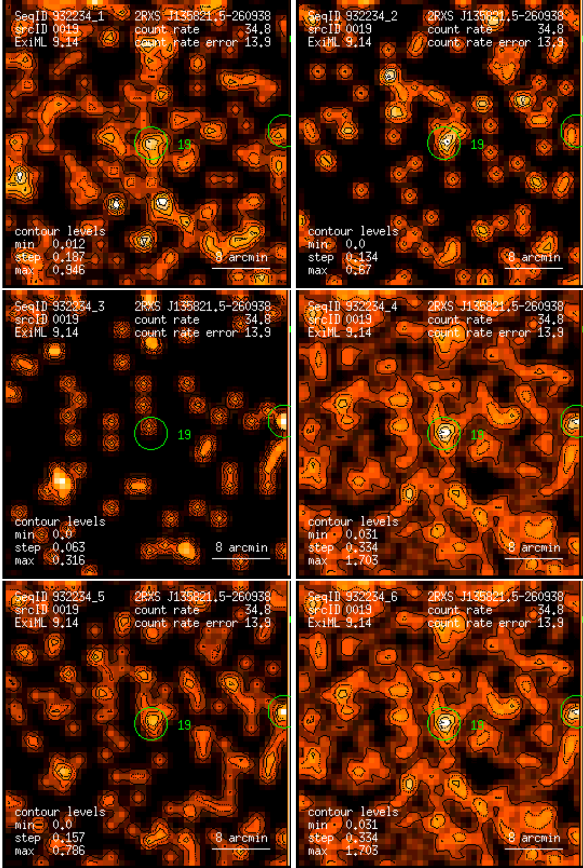
Figure 19: RASS 932234: detection 0019: band rate images, Gaussian filter: (1) PSPC channels 11 – 41, (2) 52 – 90, (3) 91 – 201, (4) 11 – 235, (5) 52 – 201, (6) 11 – 201. Broad band rates in counts/ks. Band rate contour levels in counts/ks/arcmin 2 .
