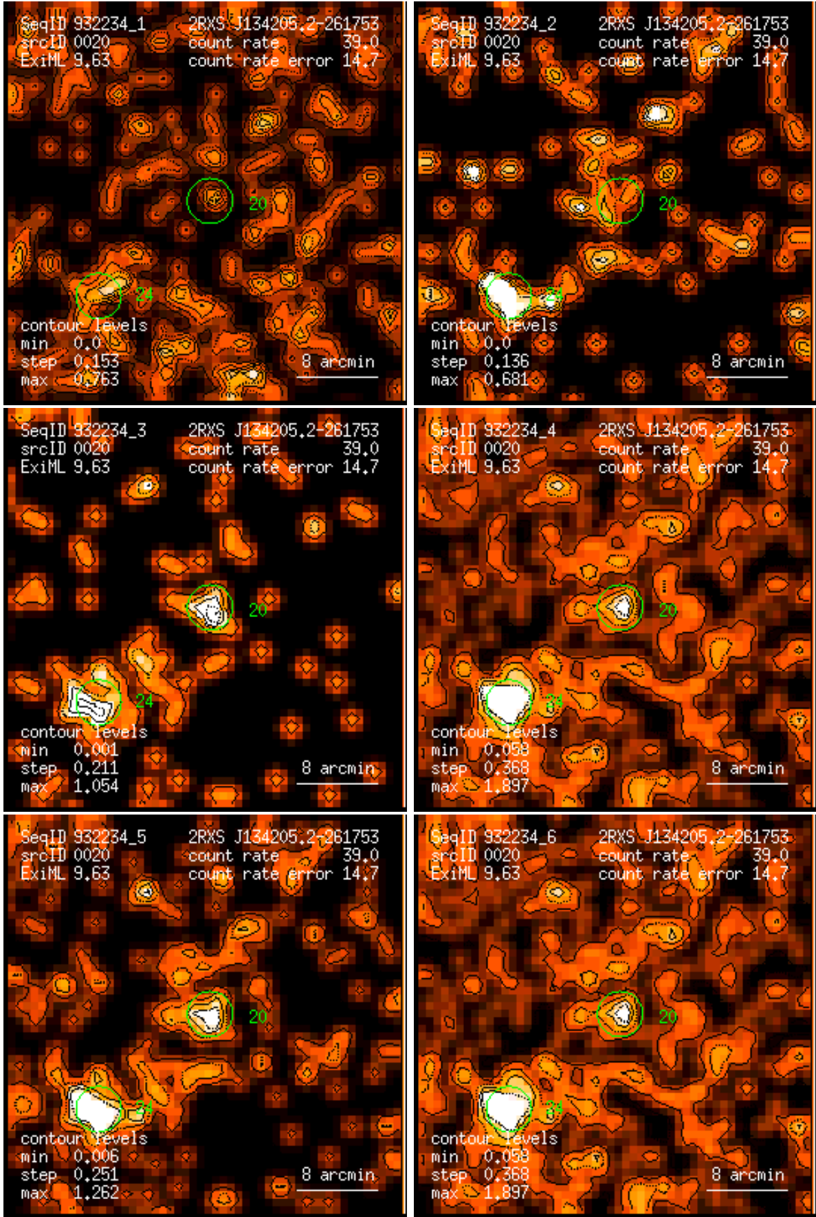
Figure 20: RASS 932234: detection 0020: band rate images, Gaussian filter: (1) PSPC channels 11 – 41, (2) 52 – 90, (3) 91 – 201, (4) 11 – 235, (5) 52 – 201, (6) 11 – 201. Broad band rates in counts/ks. Band rate contour levels in counts/ks/arcmin 2 .
