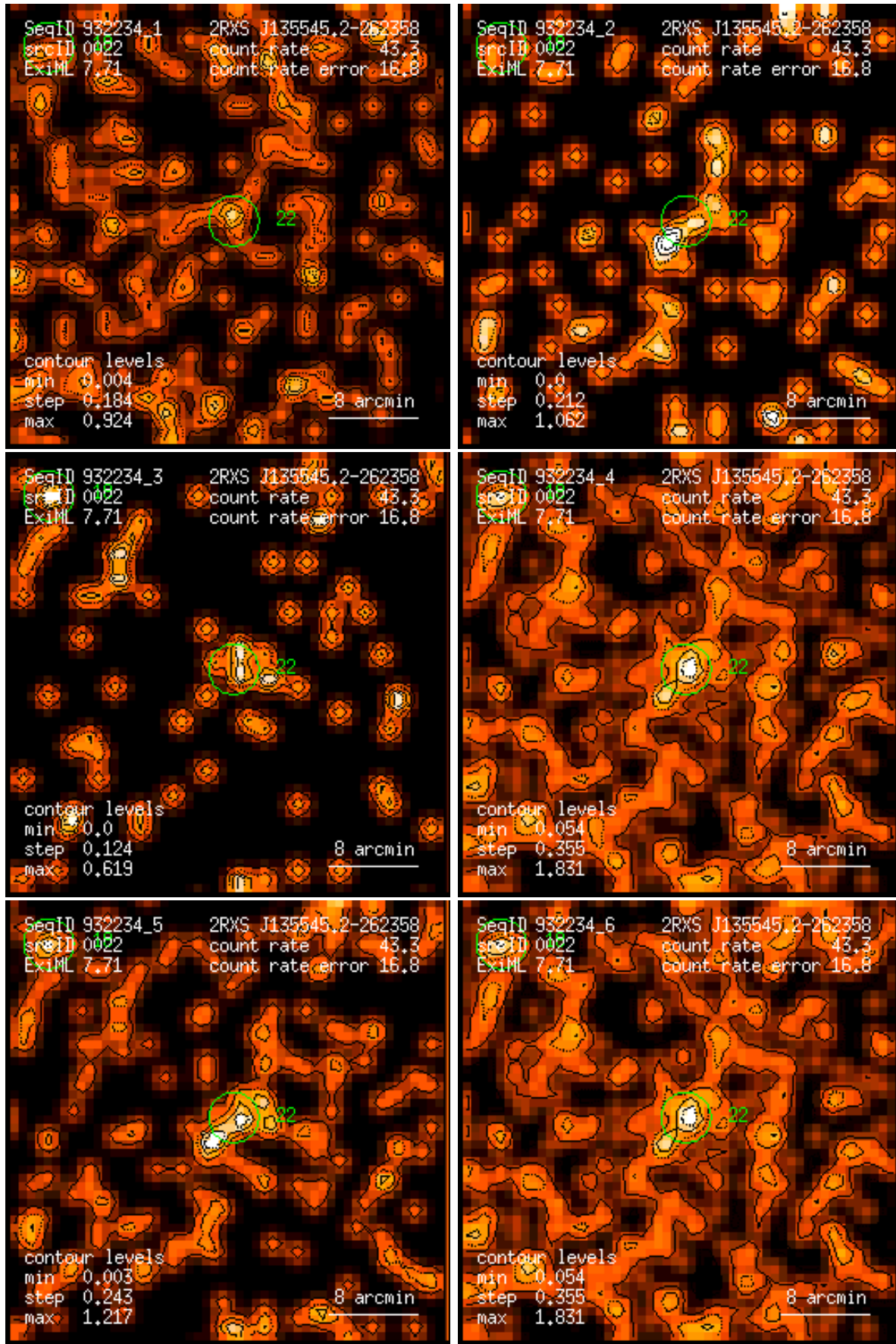
Figure 22: RASS 932234: detection 0022: band rate images, Gaussian filter: (1) PSPC channels 11 – 41, (2) 52 – 90, (3) 91 – 201, (4) 11 – 235, (5) 52 – 201, (6) 11 – 201. Broad band rates in counts/ks. Band rate contour levels in counts/ks/arcmin 2 .
