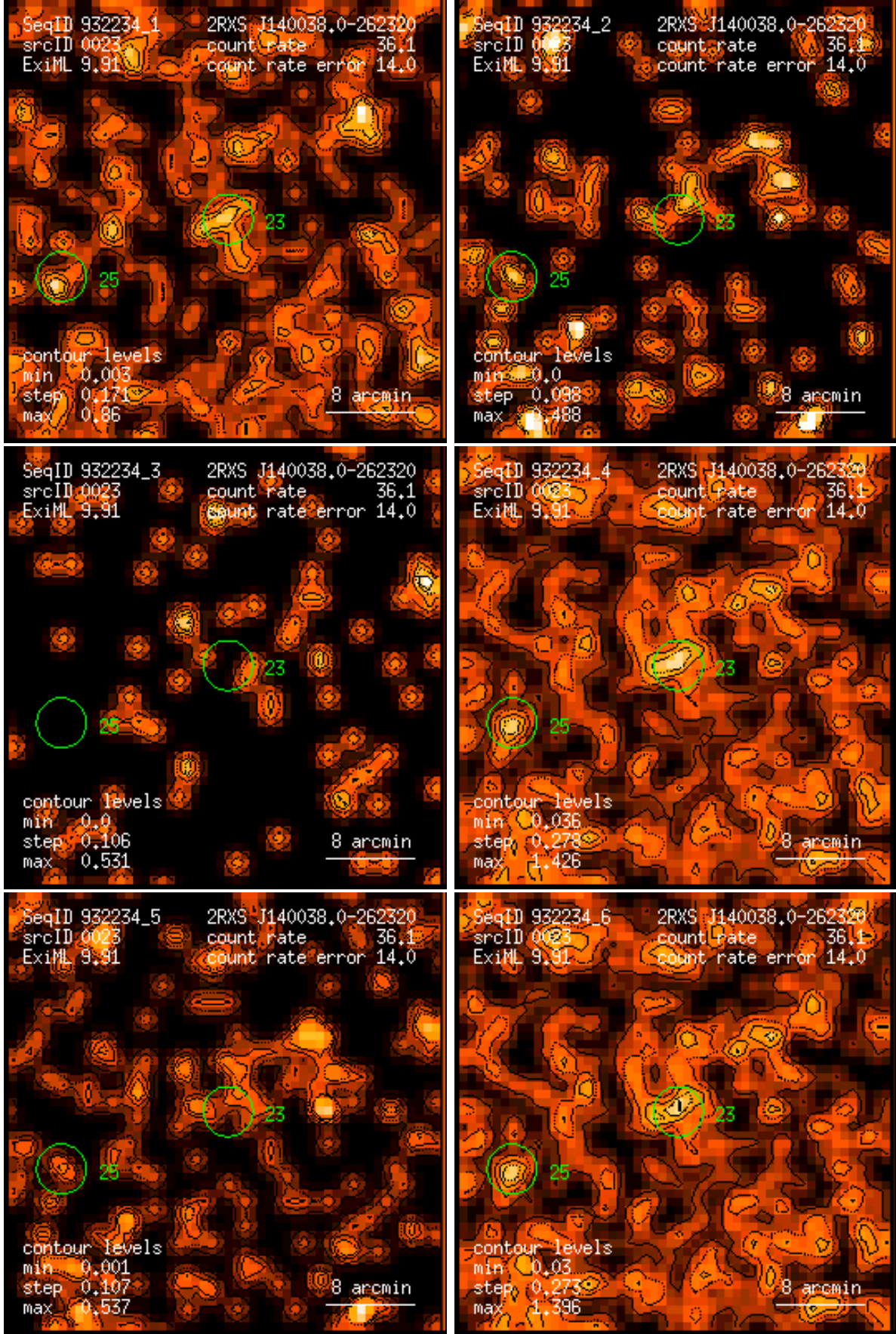
Figure 23: RASS 932234: detection 0023: band rate images, Gaussian filter: (1) PSPC channels 11 – 41, (2) 52 – 90, (3) 91 – 201, (4) 11 – 235, (5) 52 – 201, (6) 11 – 201. Broad band rates in counts/ks. Band rate contour levels in counts/ks/arcmin 2 .
