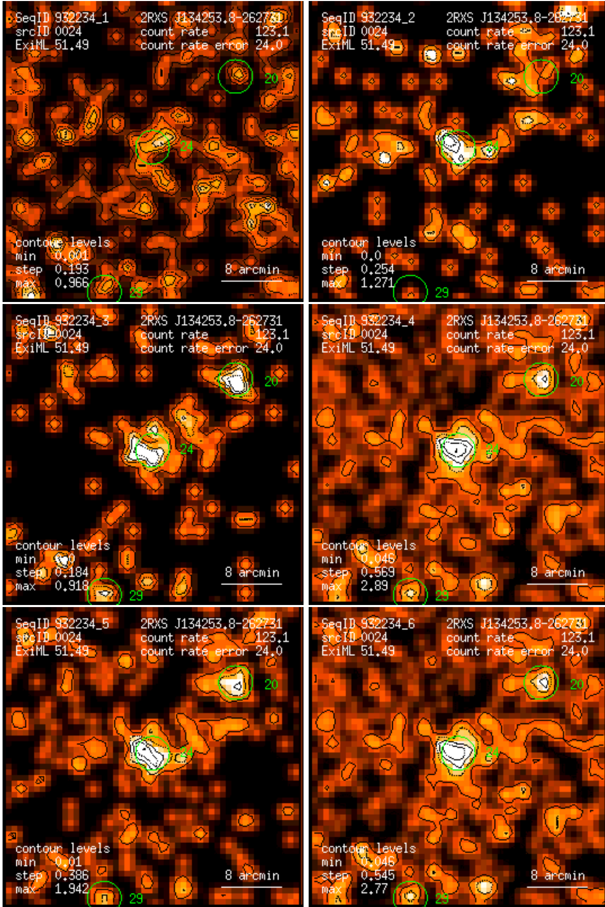
Figure 24: RASS 932234: detection 0024: band rate images, Gaussian filter: (1) PSPC channels 11 – 41, (2) 52 – 90, (3) 91 – 201, (4) 11 – 235, (5) 52 – 201, (6) 11 – 201. Broad band rates in counts/ks. Band rate contour levels in counts/ks/arcmin 2 .
