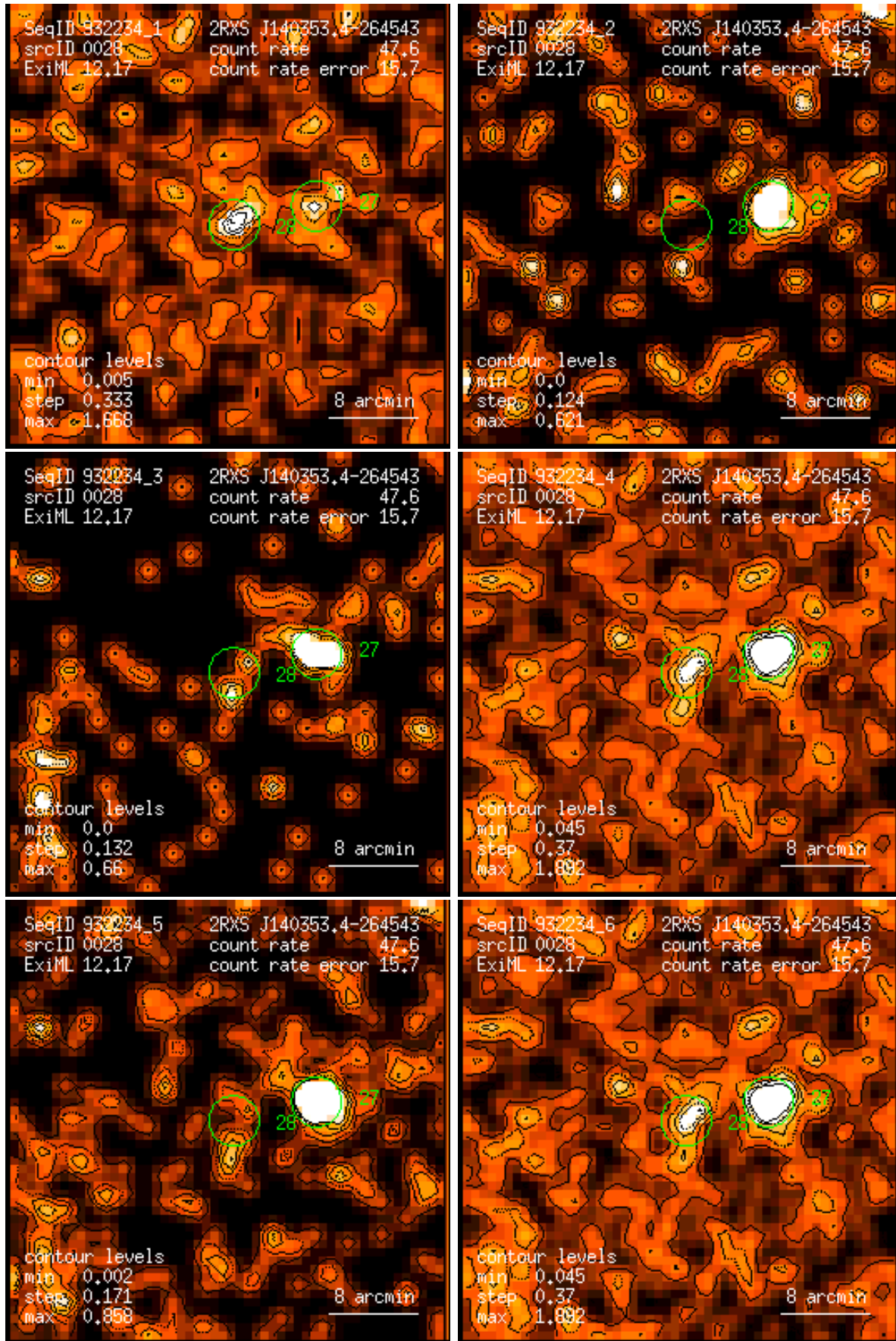
Figure 28: RASS 932234: detection 0028: band rate images, Gaussian filter: (1) PSPC channels 11 – 41, (2) 52 – 90, (3) 91 – 201, (4) 11 – 235, (5) 52 – 201, (6) 11 – 201. Broad band rates in counts/ks. Band rate contour levels in counts/ks/arcmin 2 .
