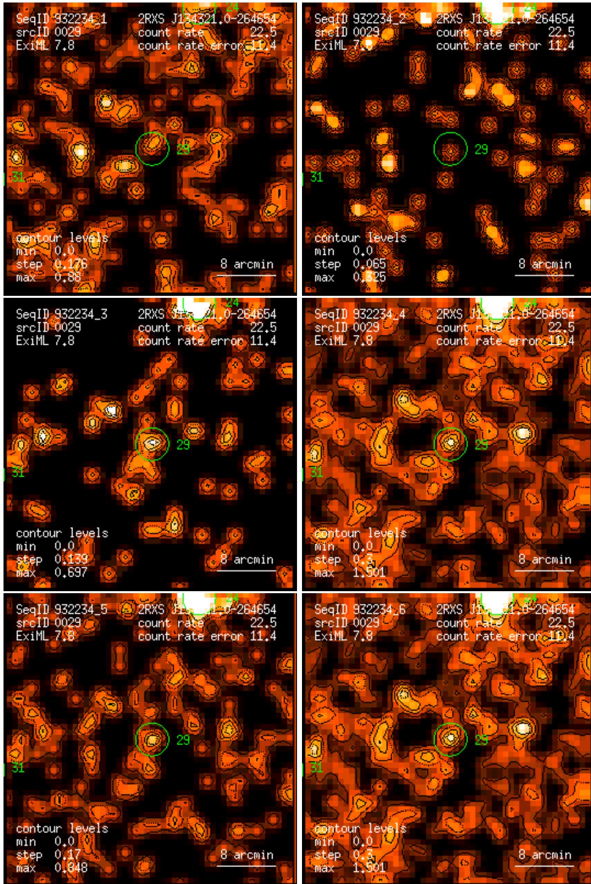
Figure 29: RASS 932234: detection 0029: band rate images, Gaussian filter: (1) PSPC channels 11 – 41, (2) 52 – 90, (3) 91 – 201, (4) 11 – 235, (5) 52 – 201, (6) 11 – 201. Broad band rates in counts/ks. Band rate contour levels in counts/ks/arcmin 2 .
