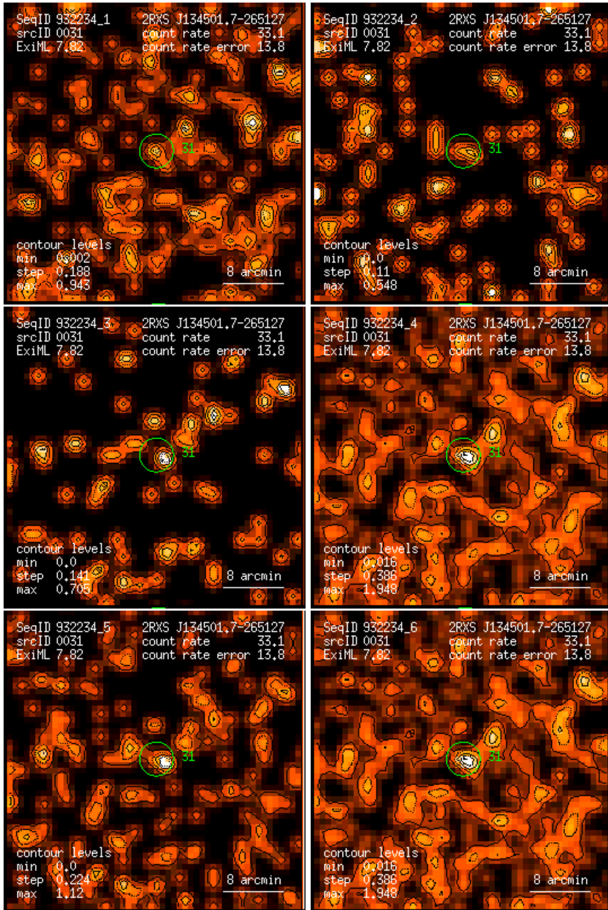
Figure 31: RASS 932234: detection 0031: band rate images, Gaussian filter: (1) PSPC channels 11 – 41, (2) 52 – 90, (3) 91 – 201, (4) 11 – 235, (5) 52 – 201, (6) 11 – 201. Broad band rates in counts/ks. Band rate contour levels in counts/ks/arcmin 2 .
