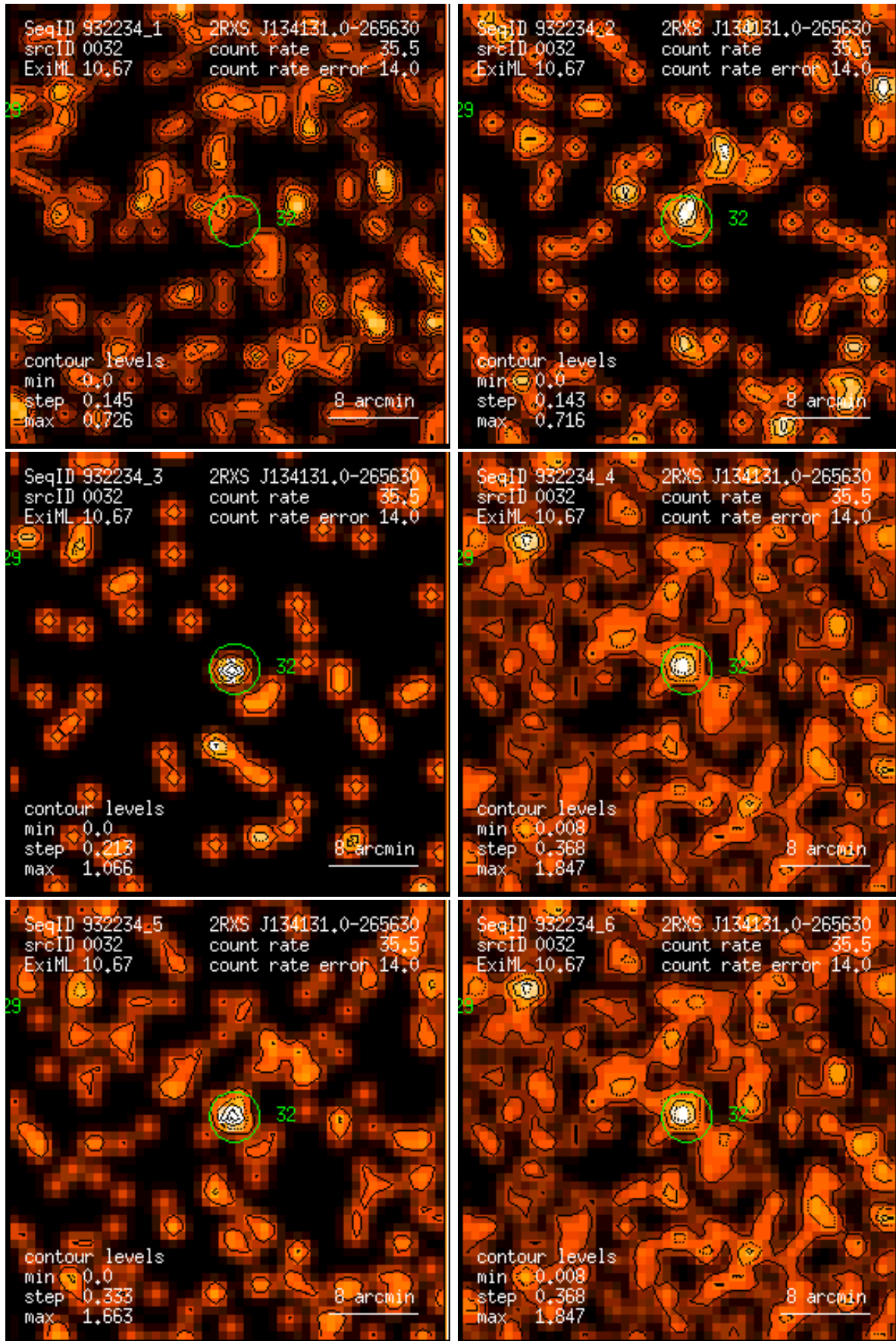
Figure 32: RASS 932234: detection 0032: band rate images, Gaussian filter: (1) PSPC channels 11 – 41, (2) 52 – 90, (3) 91 – 201, (4) 11 – 235, (5) 52 – 201, (6) 11 – 201. Broad band rates in counts/ks. Band rate contour levels in counts/ks/arcmin 2 .
