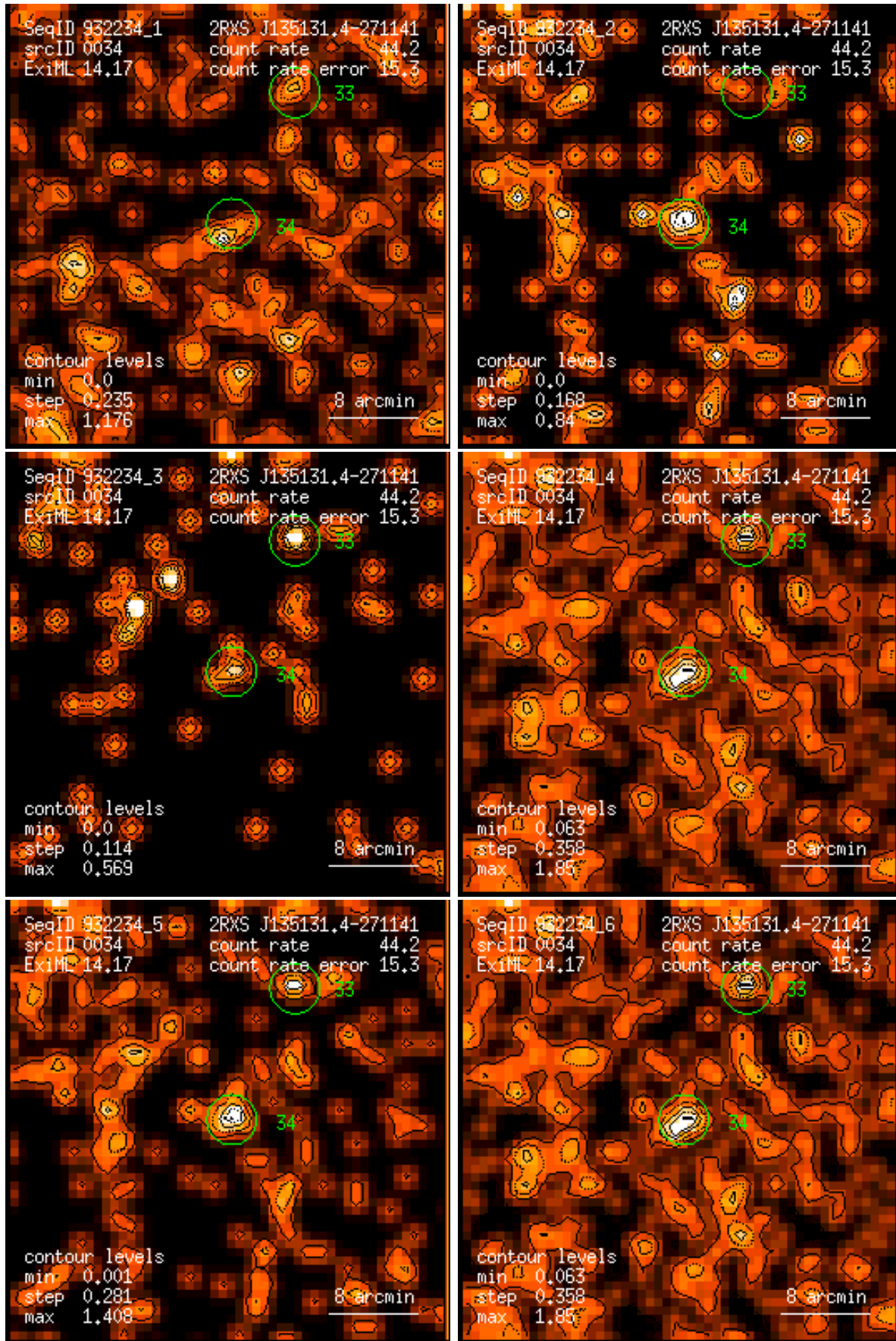
Figure 34: RASS 932234: detection 0034: band rate images, Gaussian filter: (1) PSPC channels 11 – 41, (2) 52 – 90, (3) 91 – 201, (4) 11 – 235, (5) 52 – 201, (6) 11 – 201. Broad band rates in counts/ks. Band rate contour levels in counts/ks/arcmin 2 .
