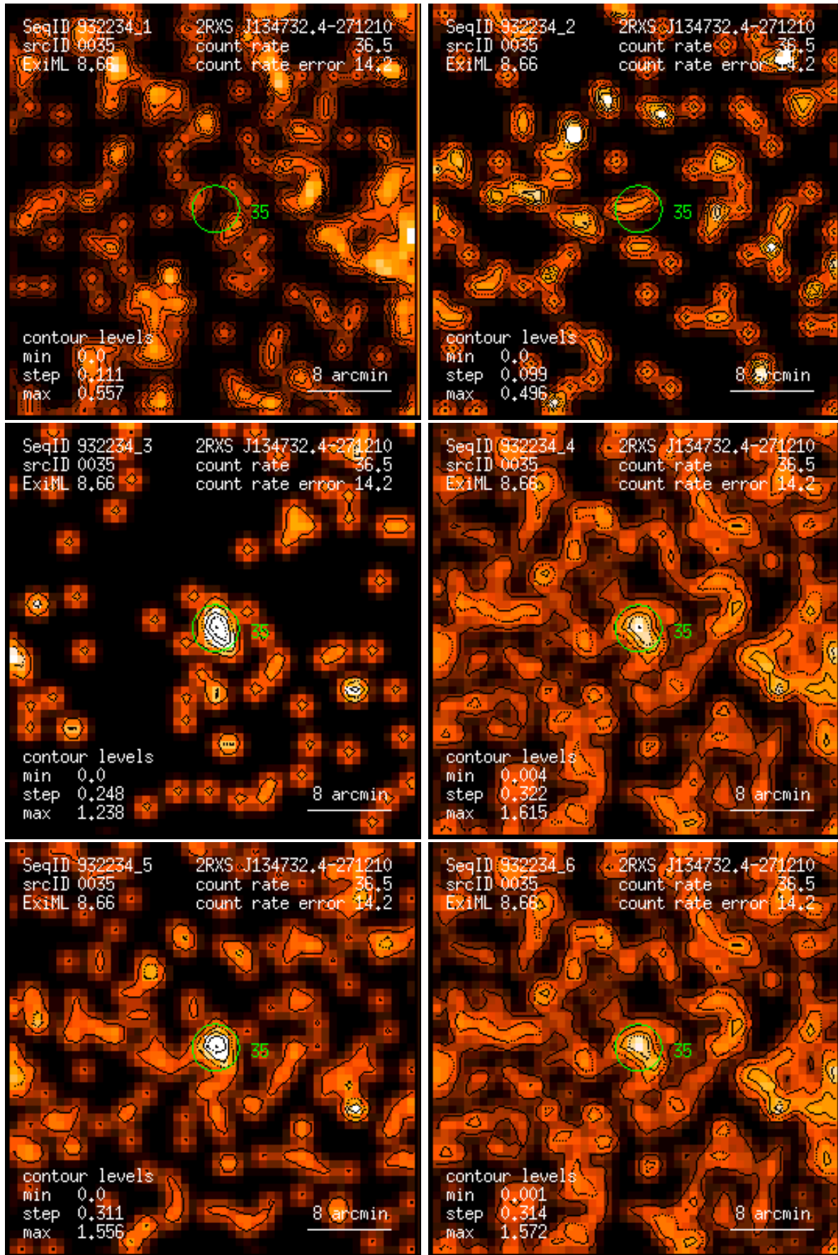
Figure 35: RASS 932234: detection 0035: band rate images, Gaussian filter: (1) PSPC channels 11 – 41, (2) 52 – 90, (3) 91 – 201, (4) 11 – 235, (5) 52 – 201, (6) 11 – 201. Broad band rates in counts/ks. Band rate contour levels in counts/ks/arcmin 2 .
