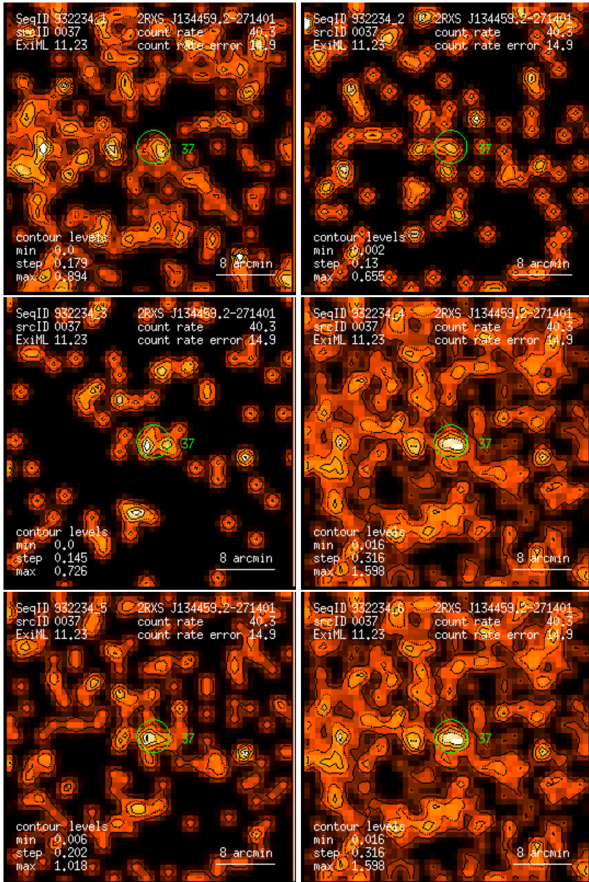
Figure 37: RASS 932234: detection 0037: band rate images, Gaussian filter: (1) PSPC channels 11 – 41, (2) 52 – 90, (3) 91 – 201, (4) 11 – 235, (5) 52 – 201, (6) 11 – 201. Broad band rates in counts/ks. Band rate contour levels in counts/ks/arcmin 2 .
