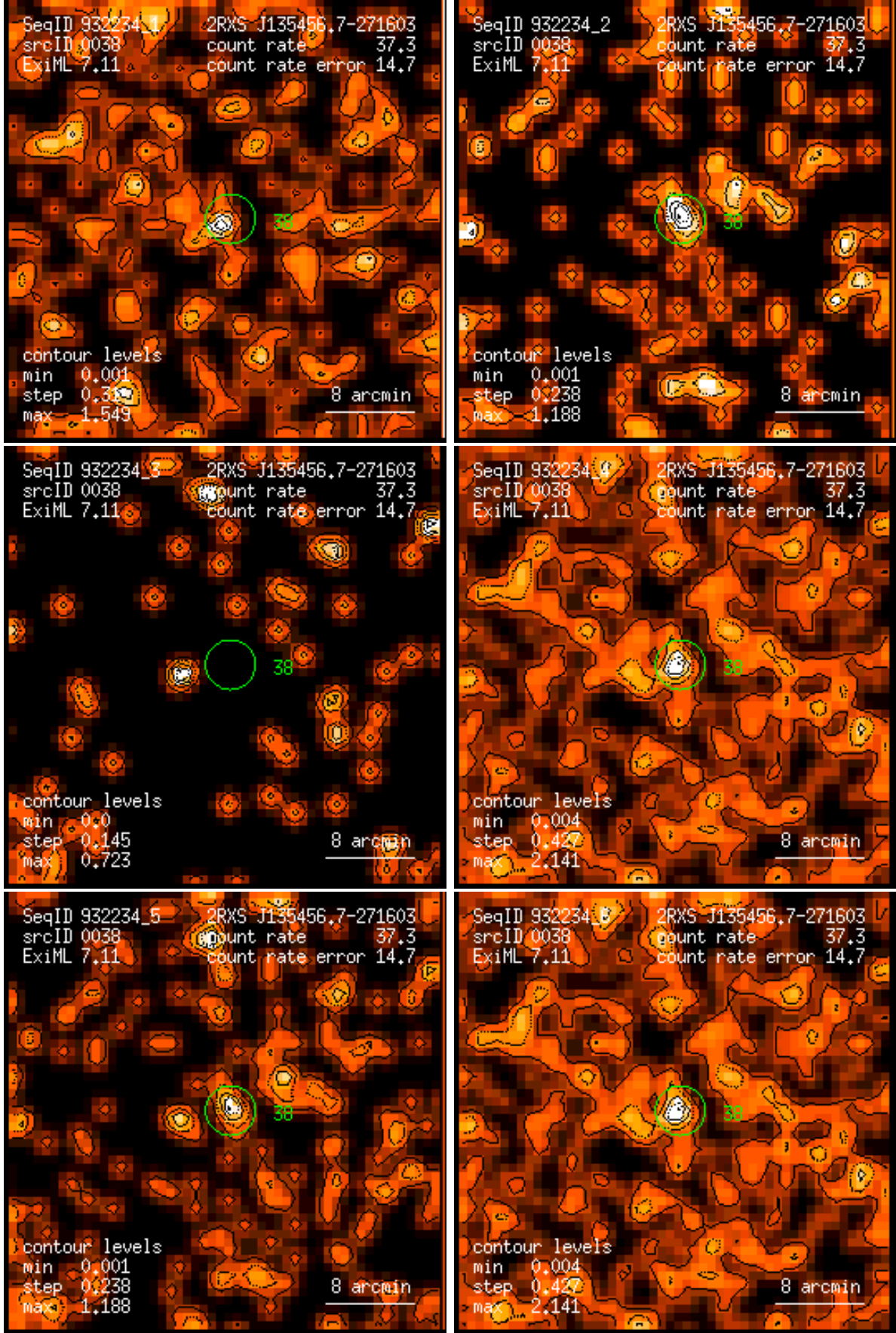
Figure 38: RASS 932234: detection 0038: band rate images, Gaussian filter: (1) PSPC channels 11 – 41, (2) 52 – 90, (3) 91 – 201, (4) 11 – 235, (5) 52 – 201, (6) 11 – 201. Broad band rates in counts/ks. Band rate contour levels in counts/ks/arcmin 2 .
