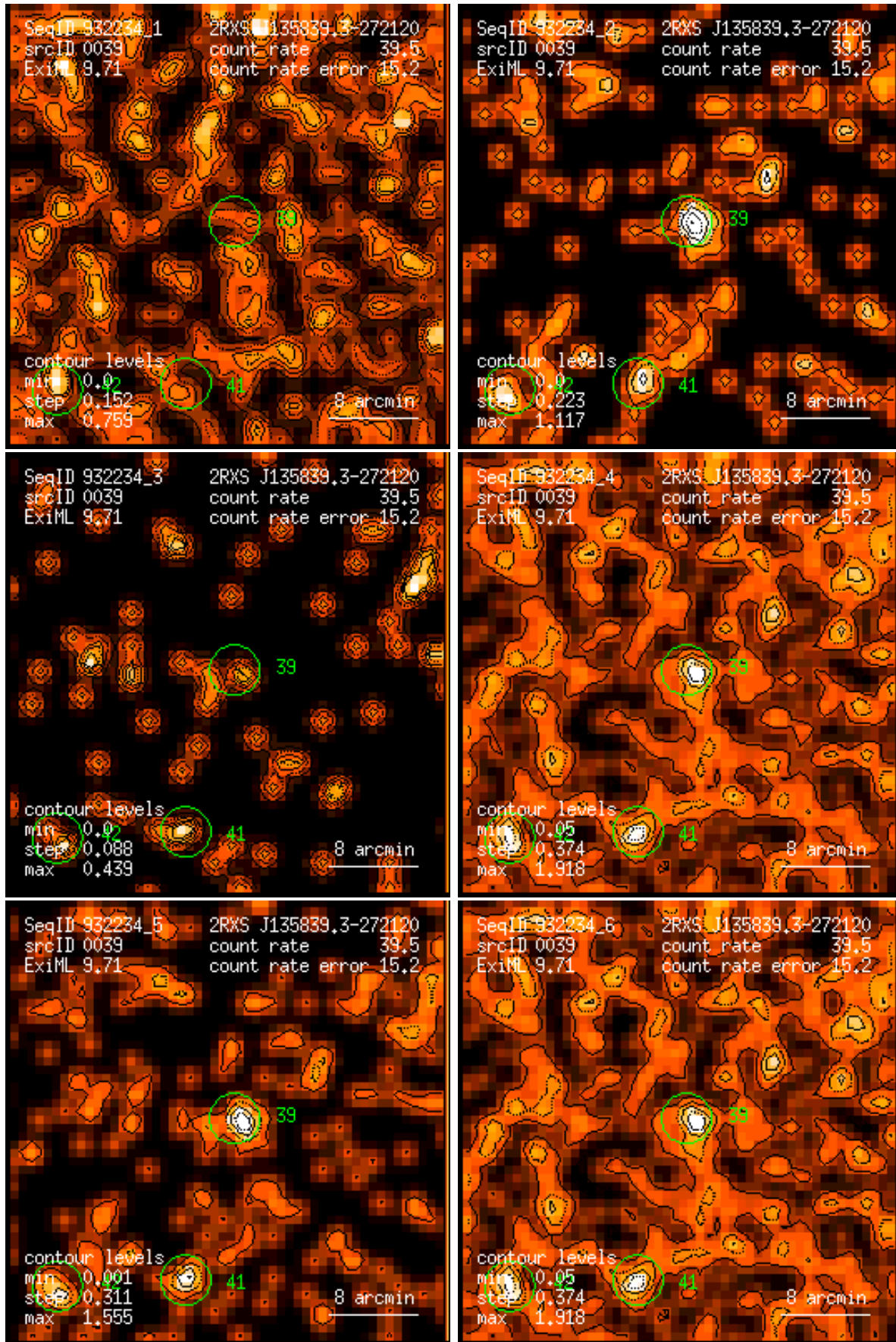
Figure 39: RASS 932234: detection 0039: band rate images, Gaussian filter: (1) PSPC channels 11 – 41, (2) 52 – 90, (3) 91 – 201, (4) 11 – 235, (5) 52 – 201, (6) 11 – 201. Broad band rates in counts/ks. Band rate contour levels in counts/ks/arcmin 2 .
