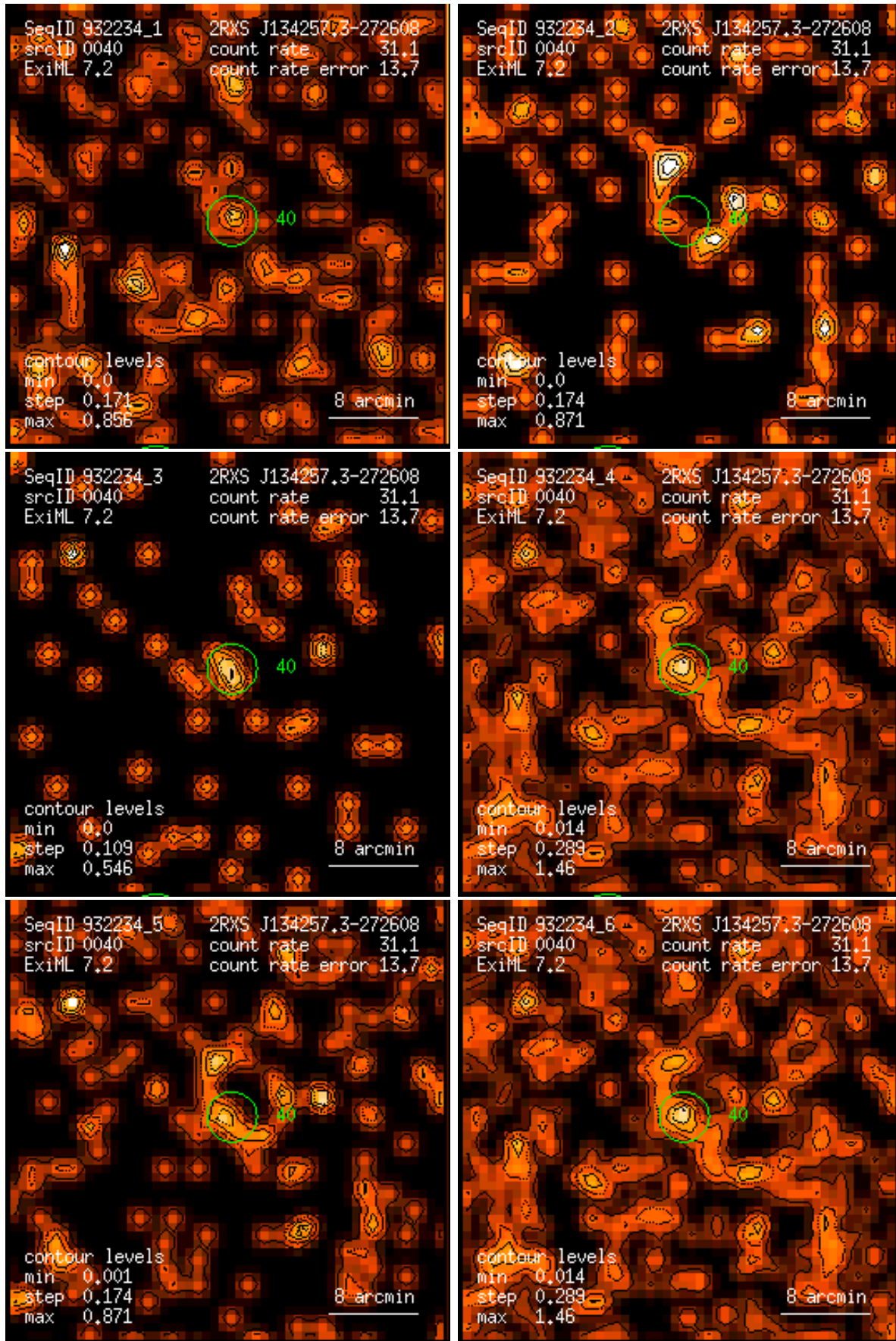
Figure 40: RASS 932234: detection 0040: band rate images, Gaussian filter: (1) PSPC channels 11 – 41, (2) 52 – 90, (3) 91 – 201, (4) 11 – 235, (5) 52 – 201, (6) 11 – 201. Broad band rates in counts/ks. Band rate contour levels in counts/ks/arcmin 2 .
