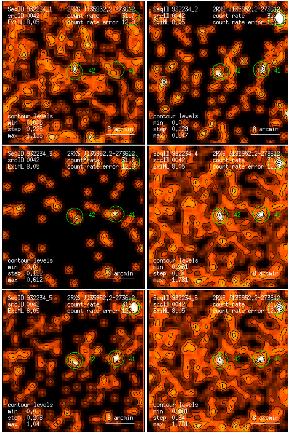
Figure 42: RASS 932234: detection 0042: band rate images, Gaussian filter: (1) PSPC channels 11 – 41, (2) 52 – 90, (3) 91 – 201, (4) 11 – 235, (5) 52 – 201, (6) 11 – 201. Broad band rates in counts/ks. Band rate contour levels in counts/ks/arcmin 2 .
