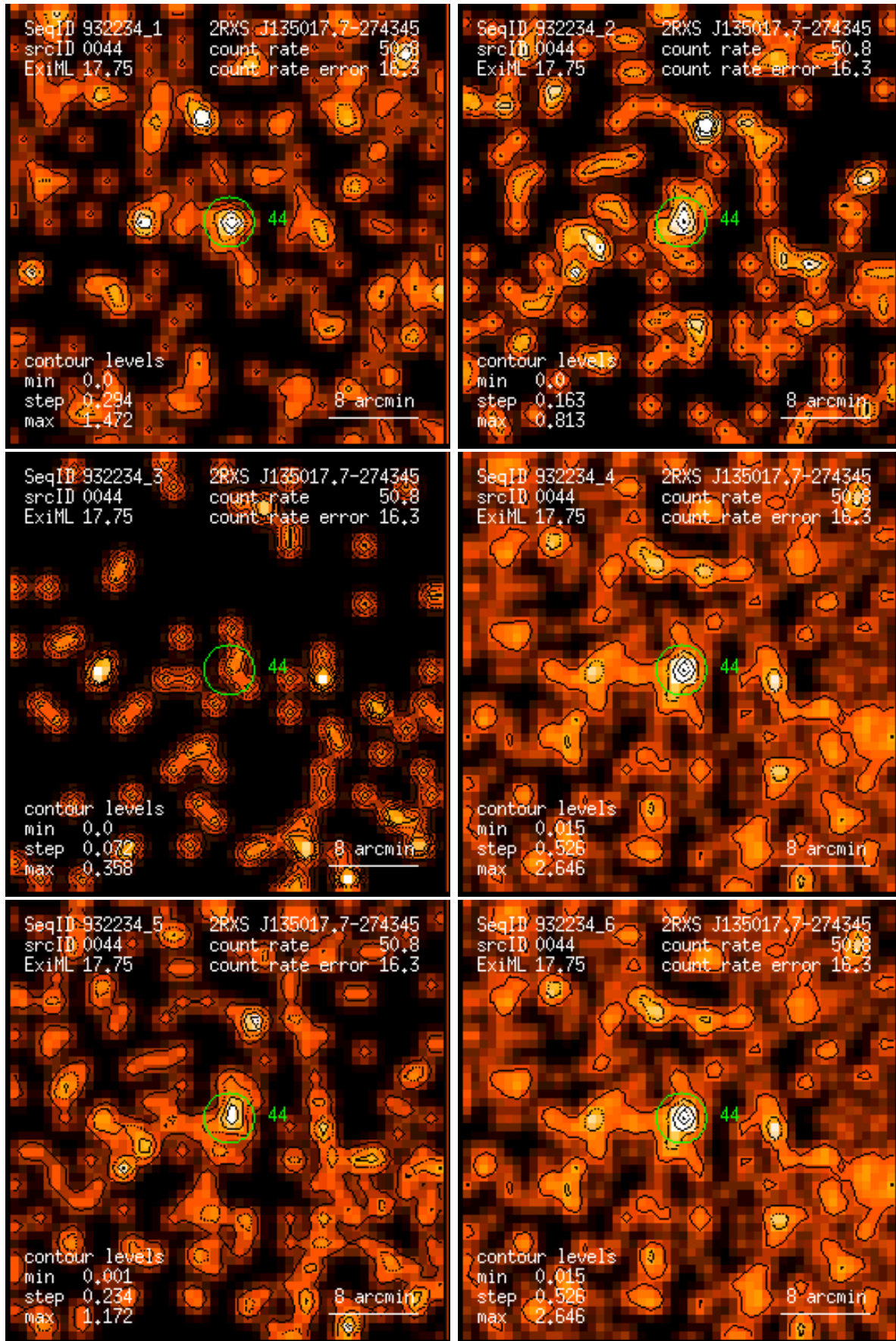
Figure 44: RASS 932234: detection 0044: band rate images, Gaussian filter: (1) PSPC channels 11 – 41, (2) 52 – 90, (3) 91 – 201, (4) 11 – 235, (5) 52 – 201, (6) 11 – 201. Broad band rates in counts/ks. Band rate contour levels in counts/ks/arcmin 2 .
